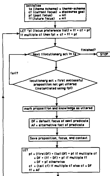
Figure 6.2. Predicate Selection Flow Chart. Selection constrained by focus.
