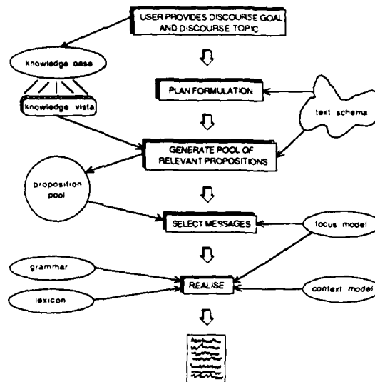
Figure 1.1. System Components and Flow of Control
