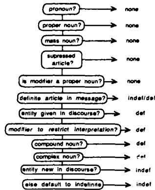
Figure 8.1. Article Selection Algorithm
