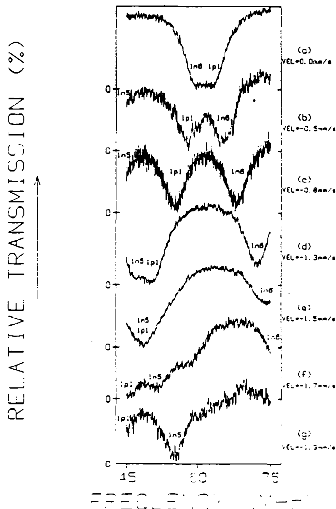
Figure 5: Typical NFMS data showing first order sidebands from the highest and lowest energy transitions of ^{57}\text{Fe} in iron, \text{ln6} and \text{lp1} respectively, a) in the vicinity of the transition center of this Zeeman split absorber. An "n" in the sideband label indicates that the sideband is at a lower energy than its parent transition, whereas a "p" indicates that the sideband is at a higher energy. As the velocity of the source is decreased b)-g), the energy of the probing radiation is decreased, and as a result the sideband from the lower energy transition, \text{lp1} , appears at lower frequencies. The sidebands from the higher energy transitions, \text{ln5} and \text{ln6} , appear separated by the excited state splitting frequency of ^{57}\text{Fe} in iron, 26 MHz.
