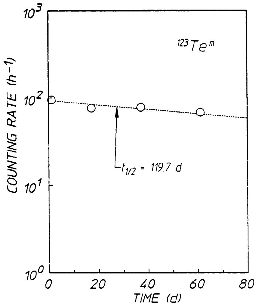
Figure 3: Plot of the time decay of the activity of the ^{123}\text{Te}^m produced in the target by irradiation with x-rays. The size of the plotted points is comparable to a 1 \sigma deviation, and the slope indicates the expected 119.7 day half-life.
