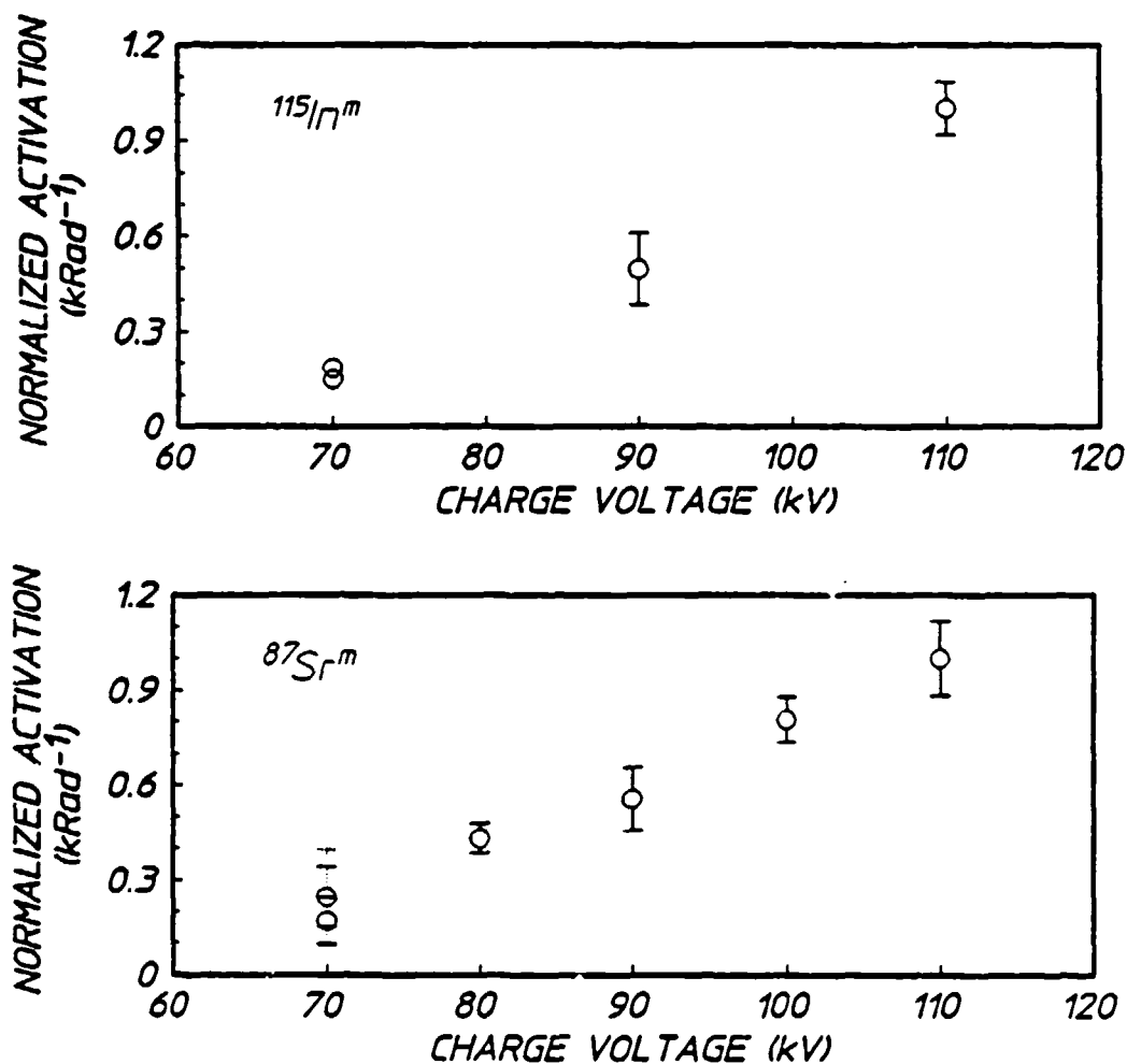
Figure 5: Isomeric activation per kilorad of dose normalized to the activation at 110 kV, as a function of the DNA/AURORA charging voltage for the following nuclei:
