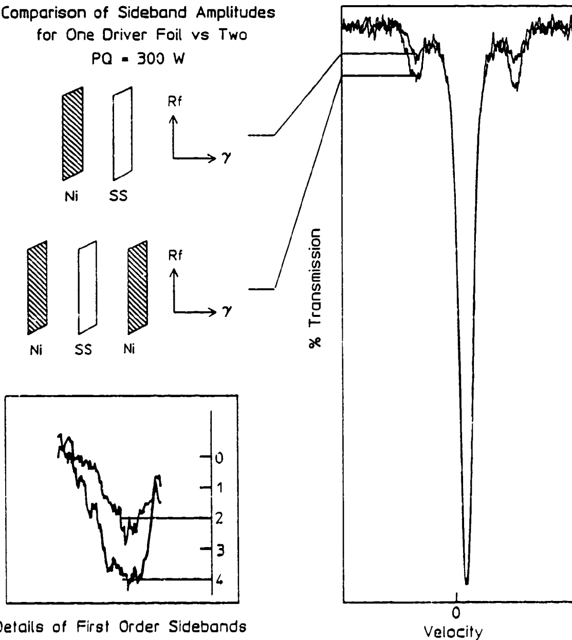
Fig. 5: Comparison of sideband amplitudes for one driver foil versus two when both are biased by a static B-field with PQ = 300 \text{ W} . Here two foils give four times the effect of one thus giving a modulation index of 4m^2 .
