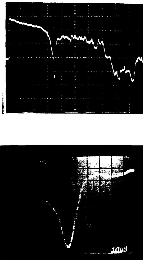
Figure E.3: Oscilloscope Photographs: Pressure Signal #2.
