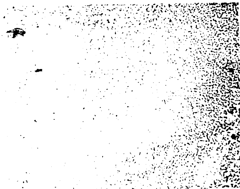
Figure 5.15 Weld metal in the middle of the weld; equiaxed dendrites (x 200).
