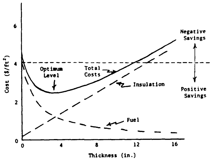
Costs of insulation as functions of thickness.
