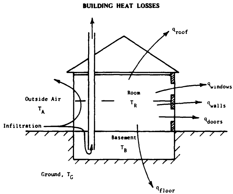
Schematic of heat flows from a building.
