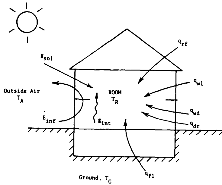
Schematic of heat gains in a building.
