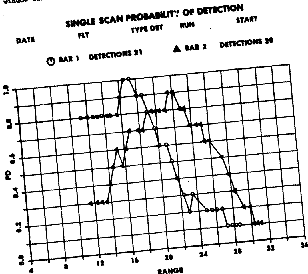
Figure 3 Single Scan Probability of Detection
