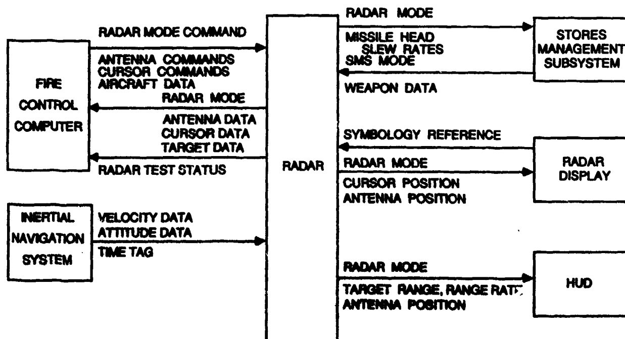
Figure 1(b) Typical Radar NUXBUS Interfaces
