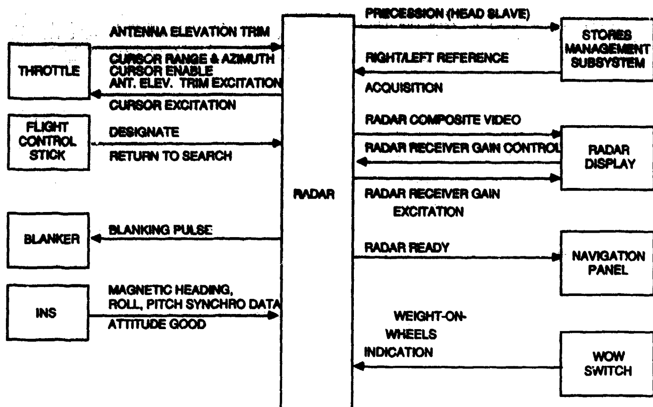
Figure 1(a) Typical Radar Discrete and Analog Signal Interfaces
