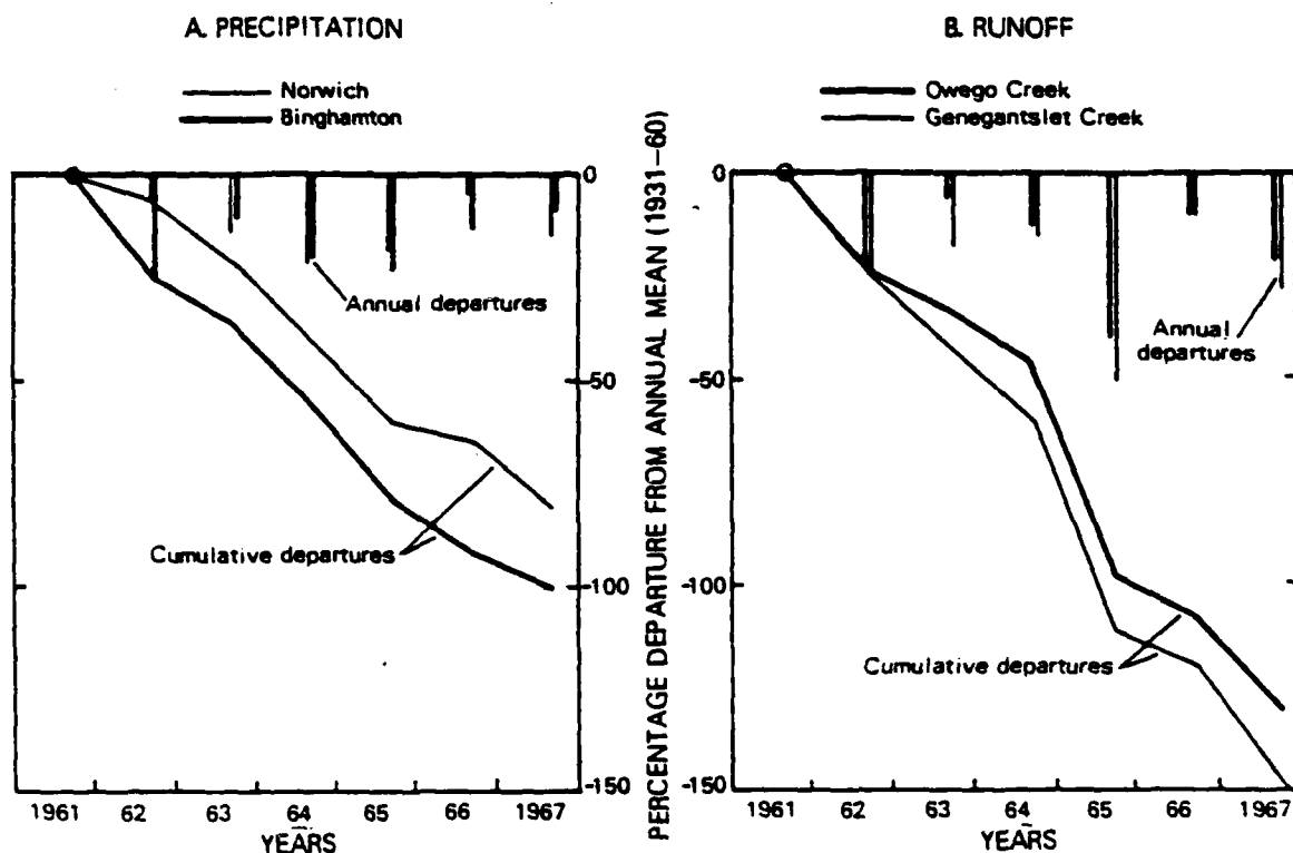
Figure C.3-1.--Departures from normal rainfall and runoff during the 1962-67 drought.
