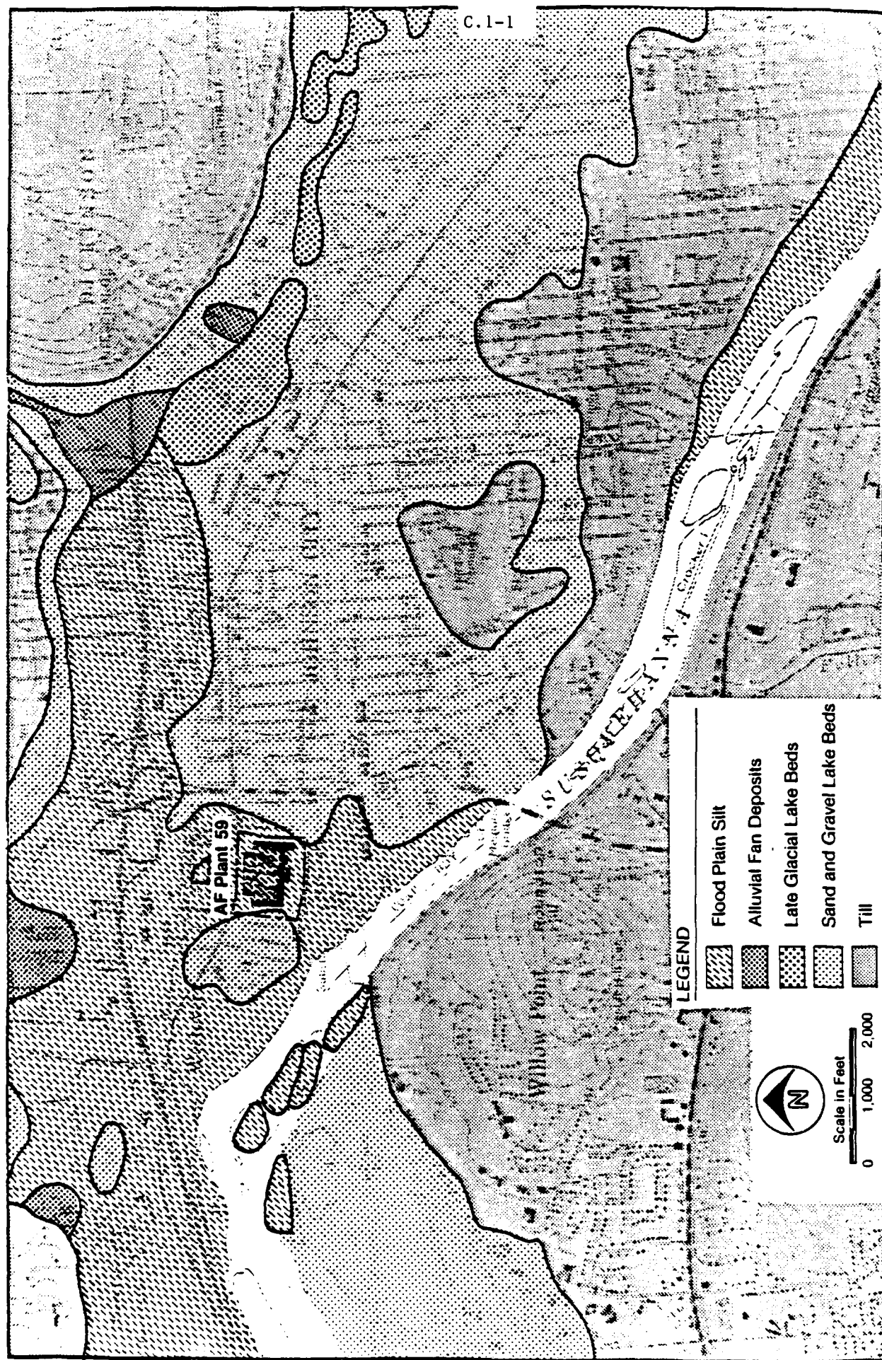
FIGURE C.1-1 Surficial Geology of Area Surrounding AF Plant 59.
