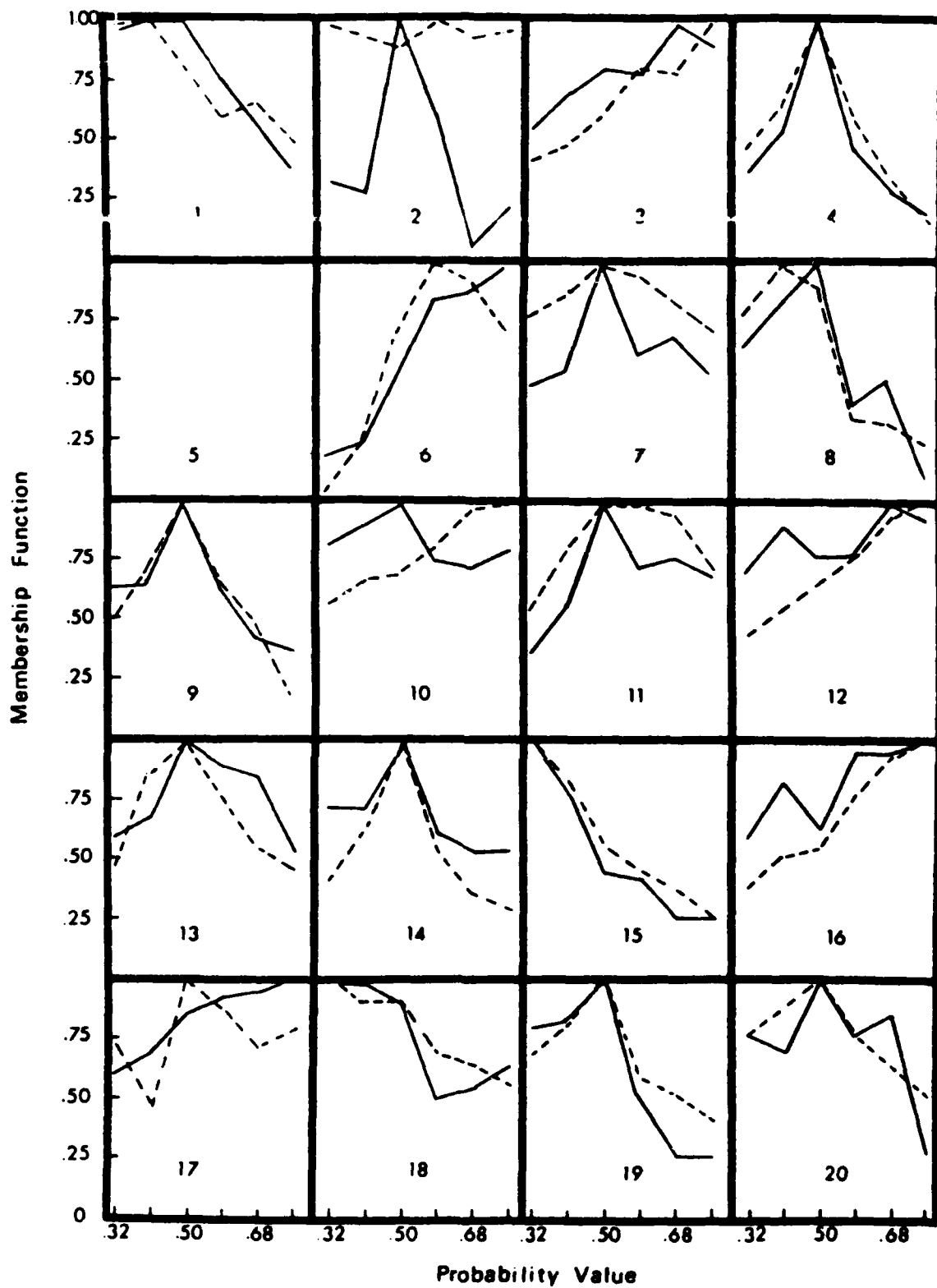
Figure 1. Individual membership functions for possible. DE functions are indicated by solid lines and PC by broken lines. Numbers in the panels refer to individual subjects.
