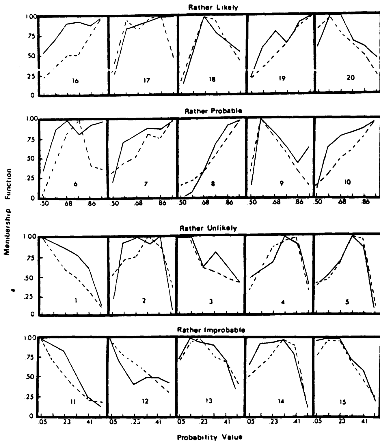
Figure 4. Individual membership functions for rather likely (subjects 16-20), rather probable (subjects 6-10), rather unlikely (subjects 1-5), and rather improbable (subjects 11-15). DE functions are indicated by solid lines and PC by broken lines.
