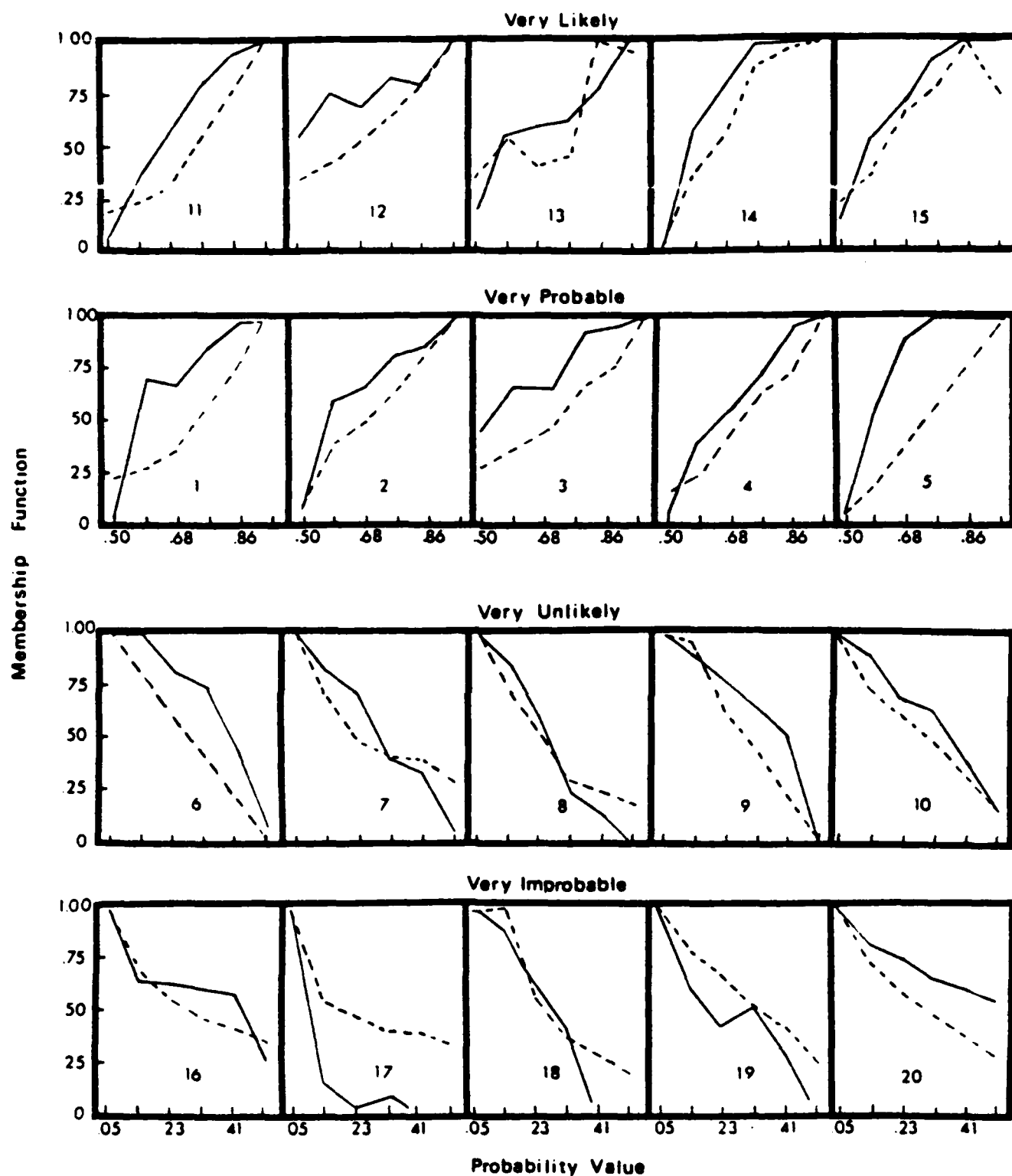
Figure 5. Individual membership functions for very likely (subjects 11-15), very probable (subjects 1-5), very unlikely (subjects 6-10), and very improbable (subjects 16-20). DE functions are indicated by solid lines and PC by broken lines.
