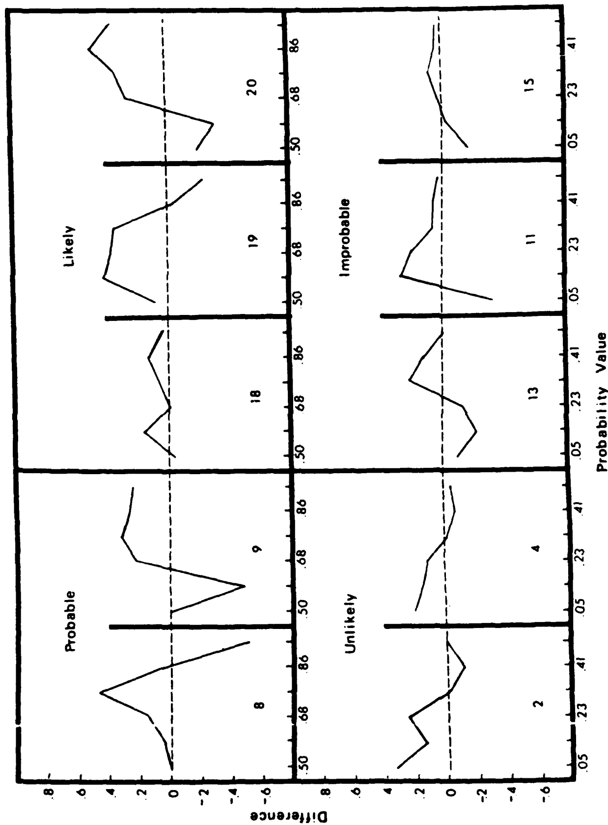
Figure 8. Empirical difference functions, \mu_W(\underline{x}) - \mu_{\text{rather}} \mu(\underline{x}) , for the 10 subjects with single peaked \mu_W(\underline{x}) .
