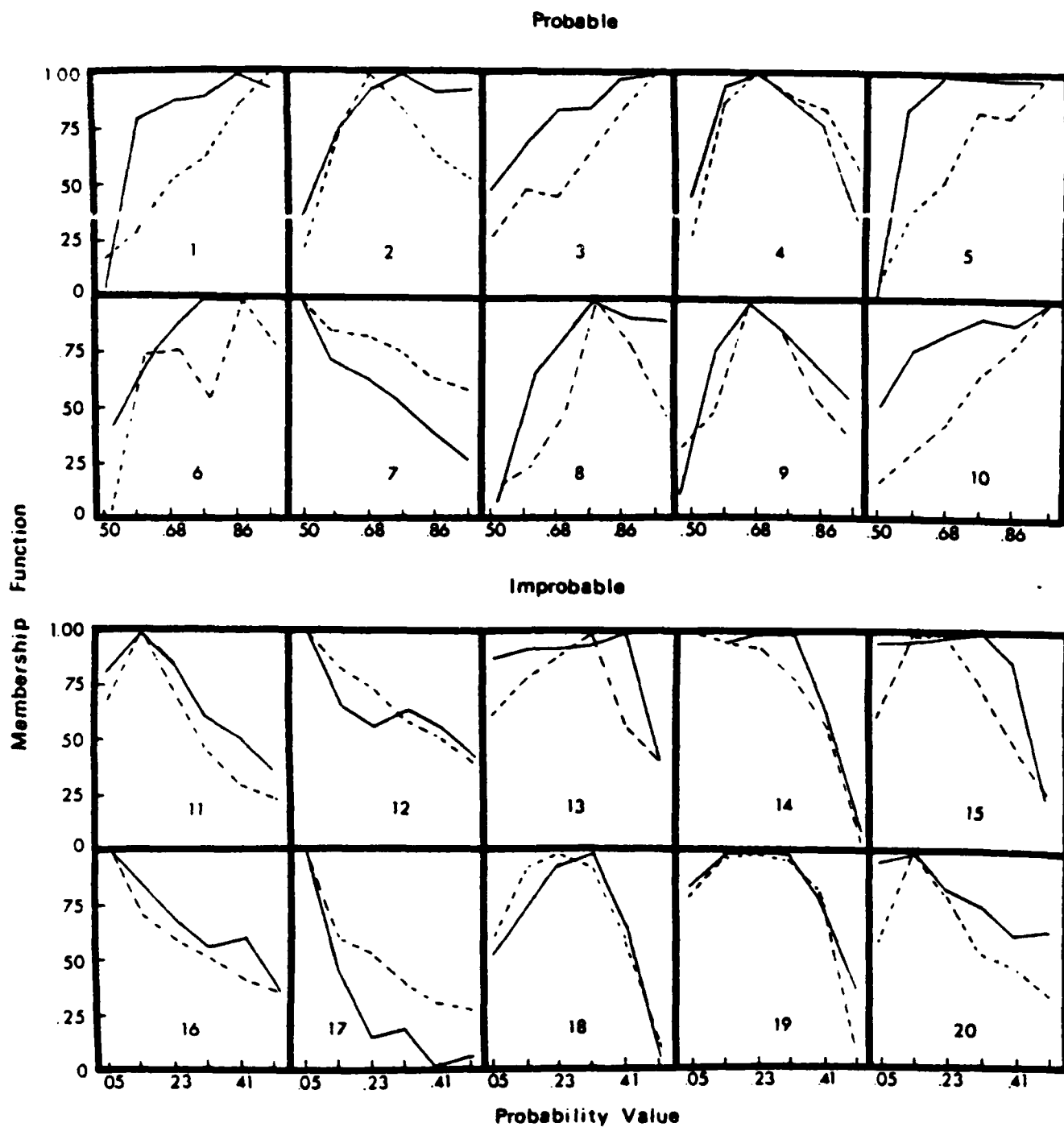
Figure 2. Individual membership functions for probable (subjects 1-10) and improbable (subjects 11-20). DE functions are indicated by solid lines and PC by broken lines.
