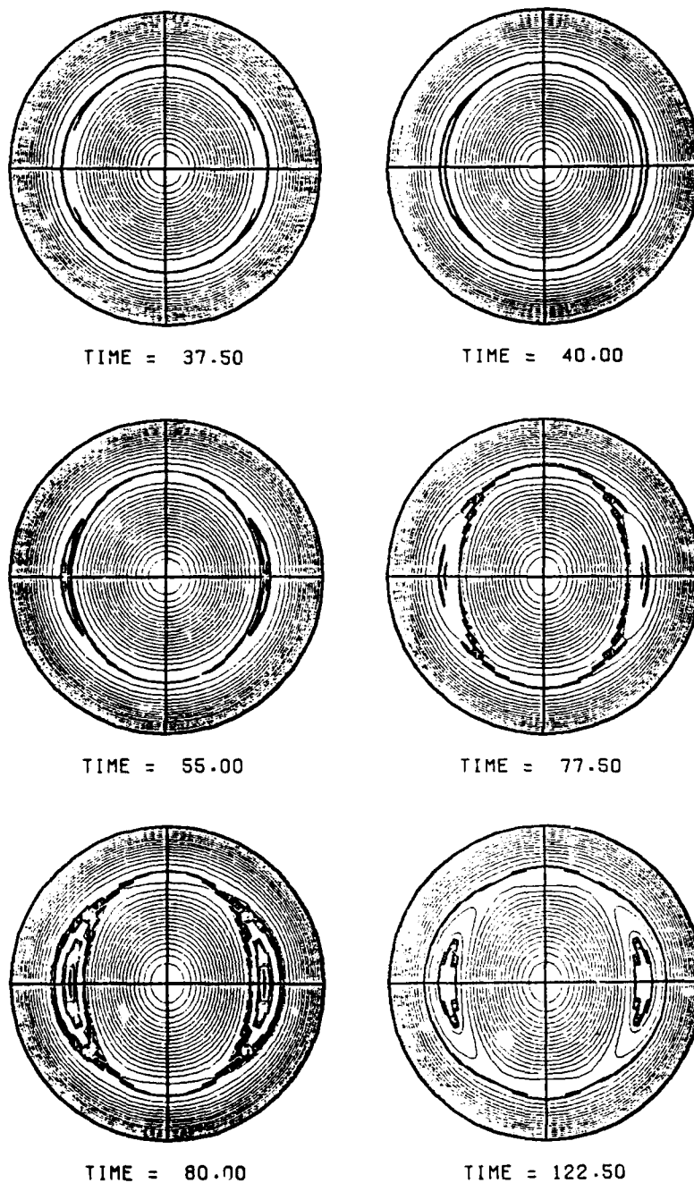
FIG.4 Time evolutions of \psi -contours and plasma surface for q_0=2.05 . Formation of vacuum bubbles is observed for plasma of q_0 \geq 2 with finite \kappa_1 .
