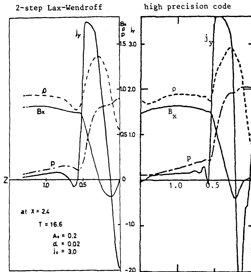
Fig.2. Cross sectional distributions of the current ( j_y ), x component of the magnetic field ( B_x ), pressure ( p ), and density ( \rho ) on a plane at x = 2.4 . Note the opposite changes of B_x and p (and \rho ) across the current layer, thus showing evidence of slow shocks.
