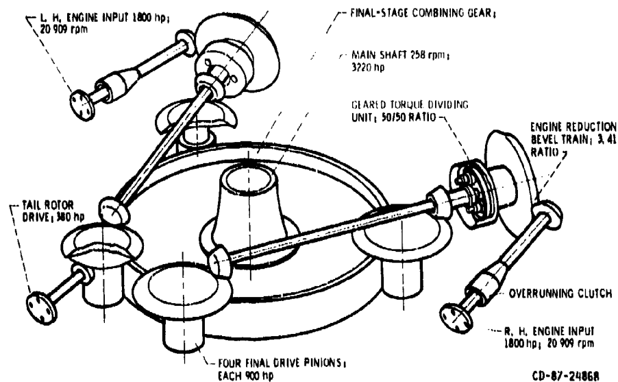
(a) 3600-hp SPLIT TORQUE.
