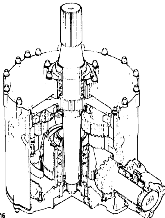
(c) 500-hp BEARINGLESS PLANETARY (LOW-RATIO).
