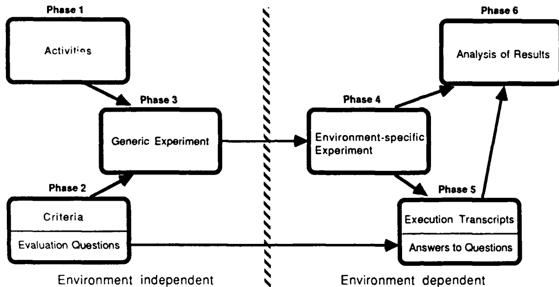
Figure 2-1: Phases and Products in the Evaluation Methodology
