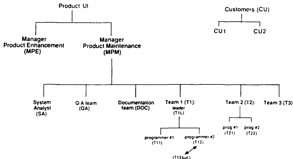
Figure 7-2: Organizational Structure
