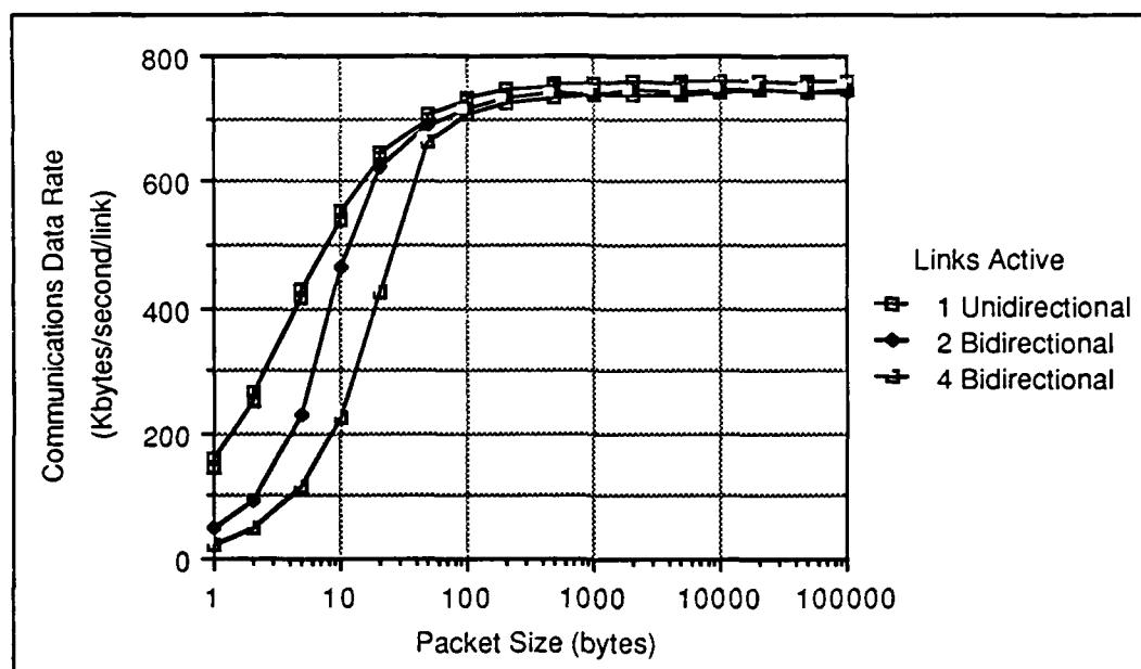
Figure 3.4. T414 Packet Size Effects on Communication Rate
