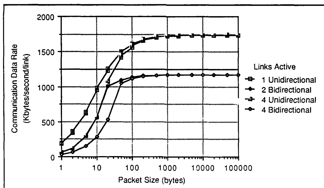
Figure 3.5. T800 Packet Size Effects on Communication Rate
