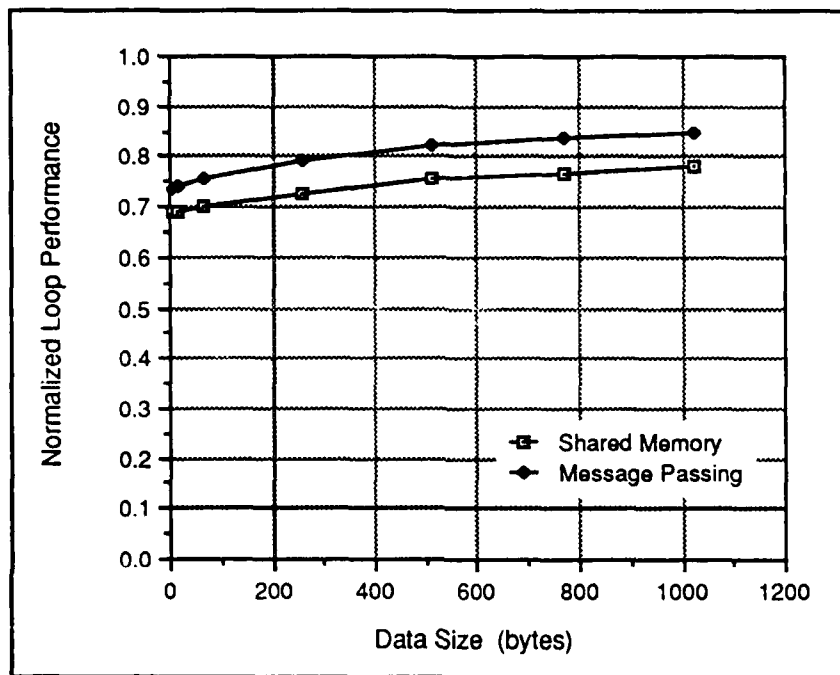
Figure 5.8. Intermediate Process Degradation During Communication
