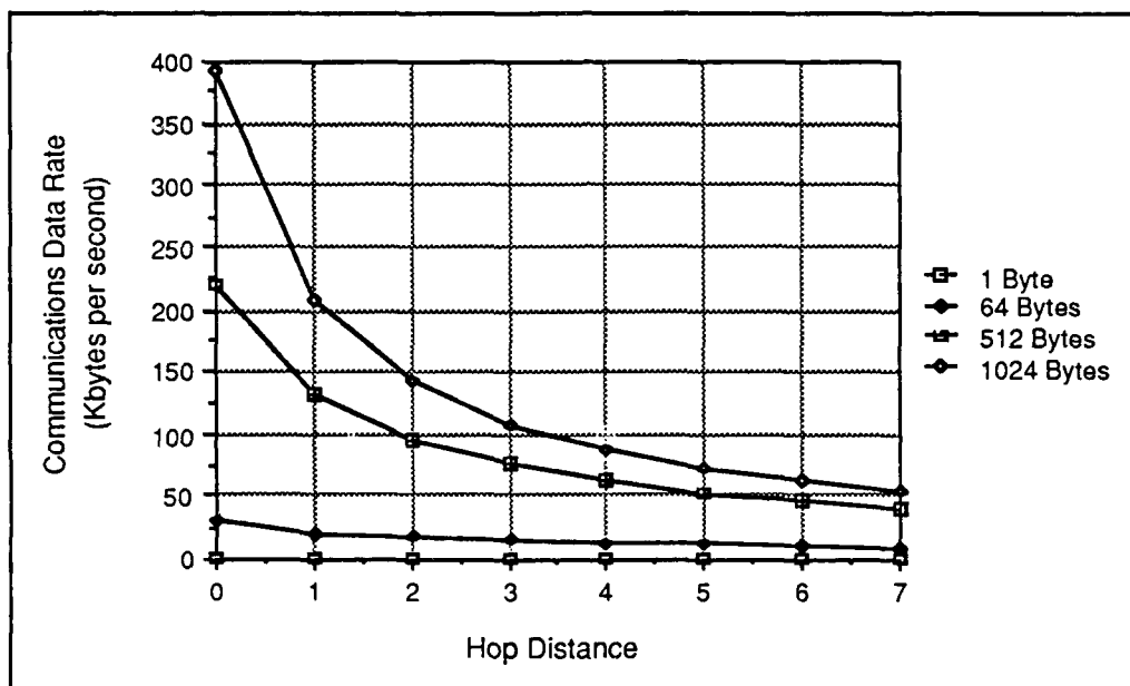
Figure 4.12. Hop Distance Effects on Communication Data Rate
