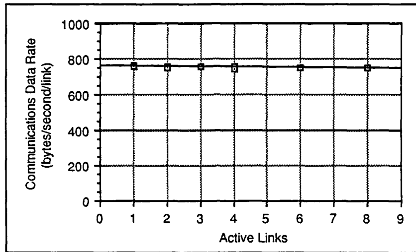
Figure 3.2. T414 Multiple Link Effects on Communications Rate
