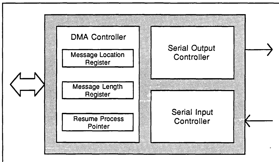
Figure 2.6. Hardware Communication Link Logical Block Diagram
