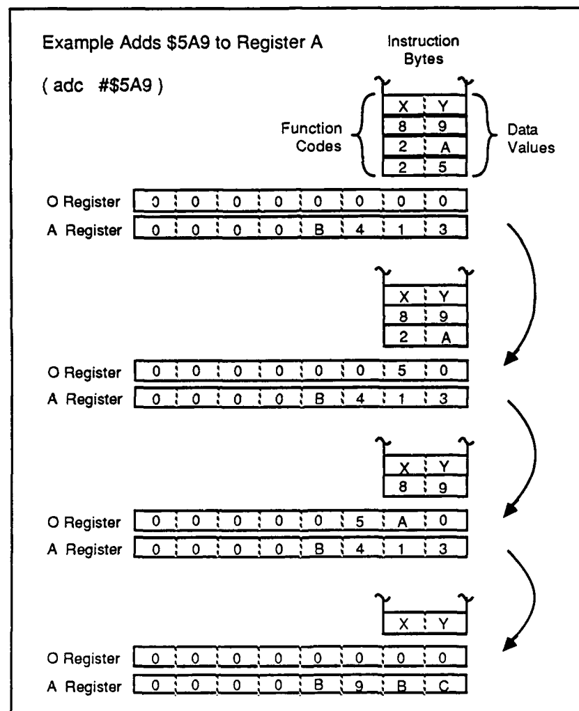
Figure 2.5. Example of Operand Register Operation
