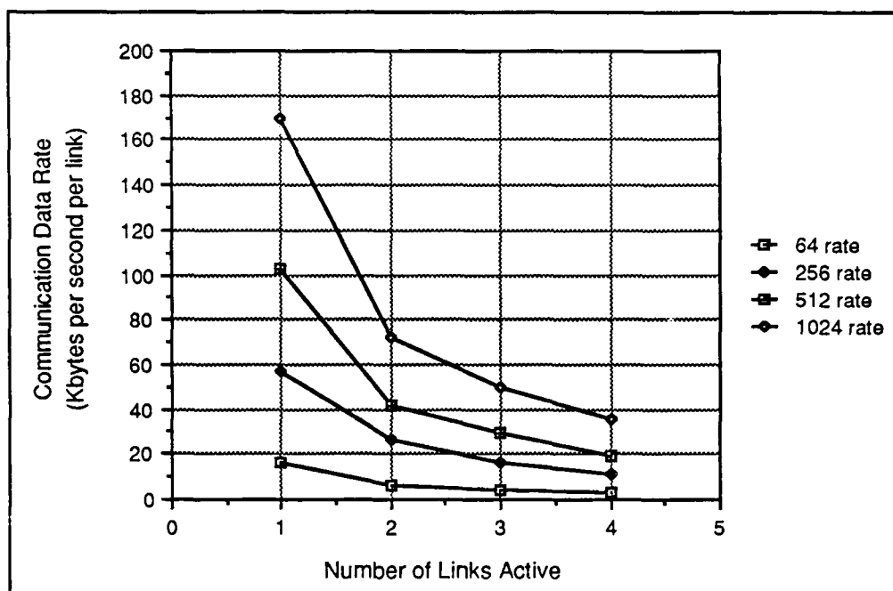
Figure 4.15. Multiple Hardware Link Communications Rates
