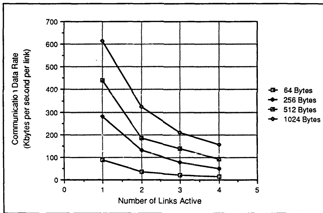
Figure 5.10. Multiple Hardware Link Communication Rates
