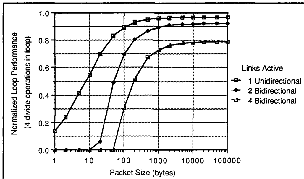
Figure 3.9. T800 Performance Degradation with Four Divide Operations
