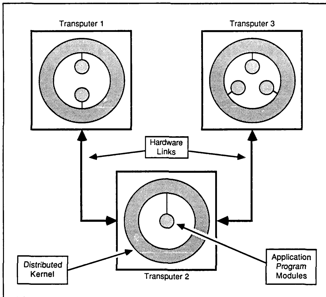
Figure 4.1. Physical Configuration of Shared Memory Kernel
