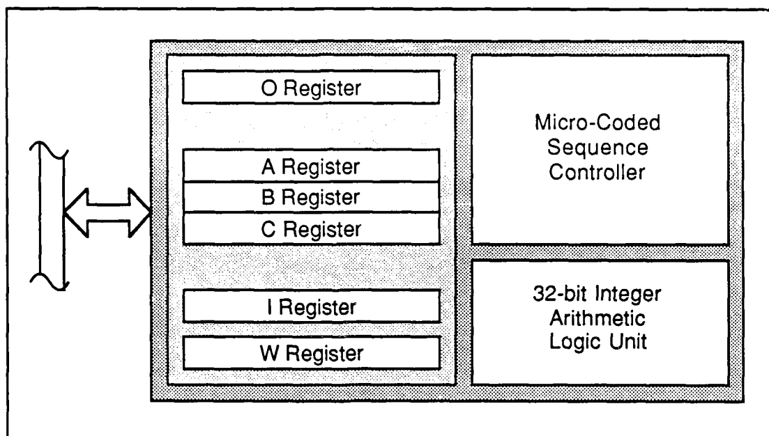
Figure 2.4. Processor Block Diagram
