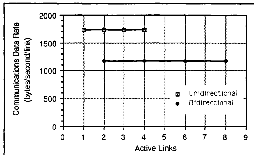
Figure 3.3. T800 Multiple Link Effects on Communications Rate
