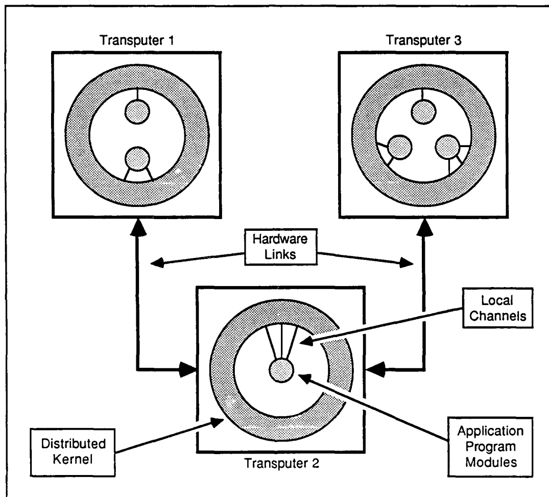
Figure 5.1. Physical Configuration of Message-Passing Kernel
