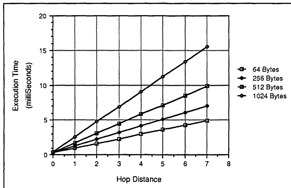
Figure 4.10. Get Operation Timing Test Results
