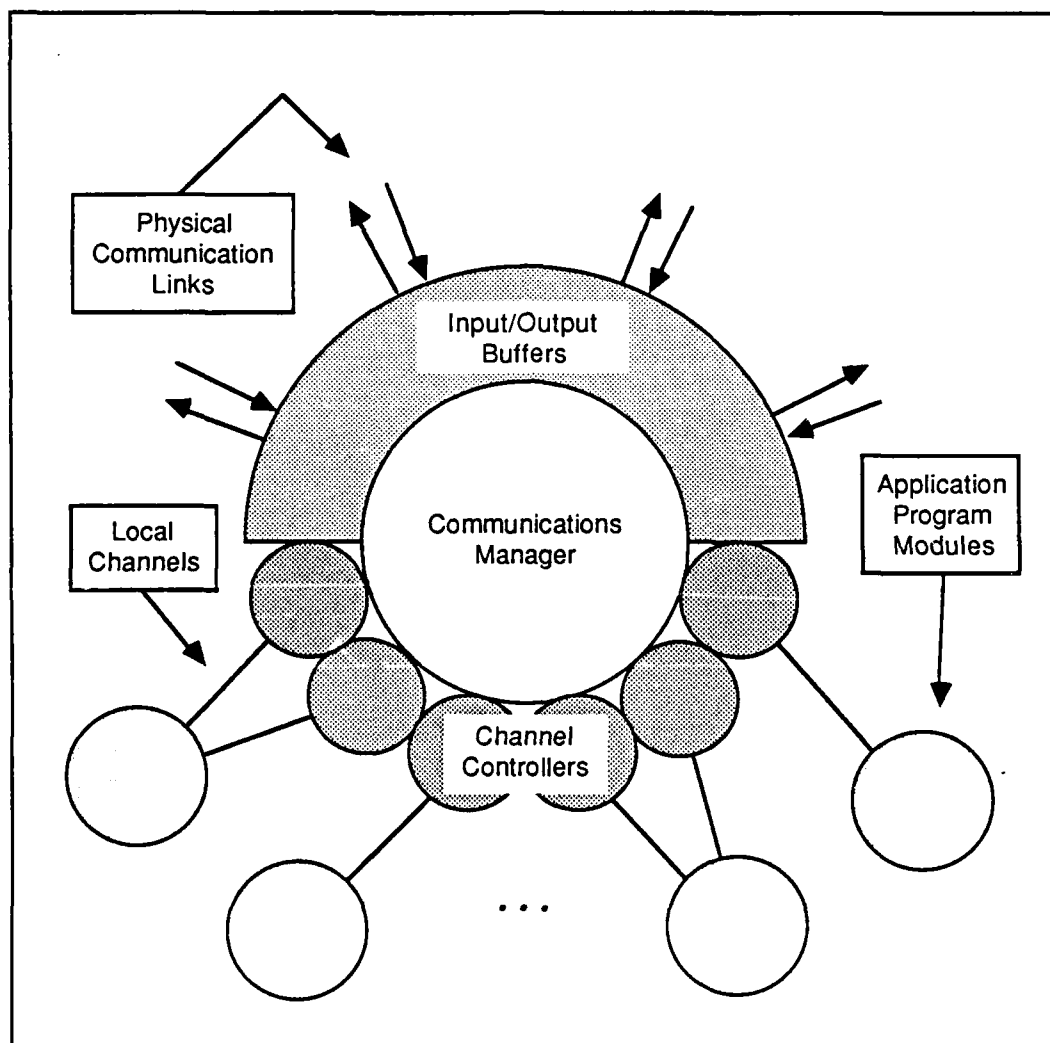
Figure 5.3. Message Passing Kernel Logical Block Diagram
