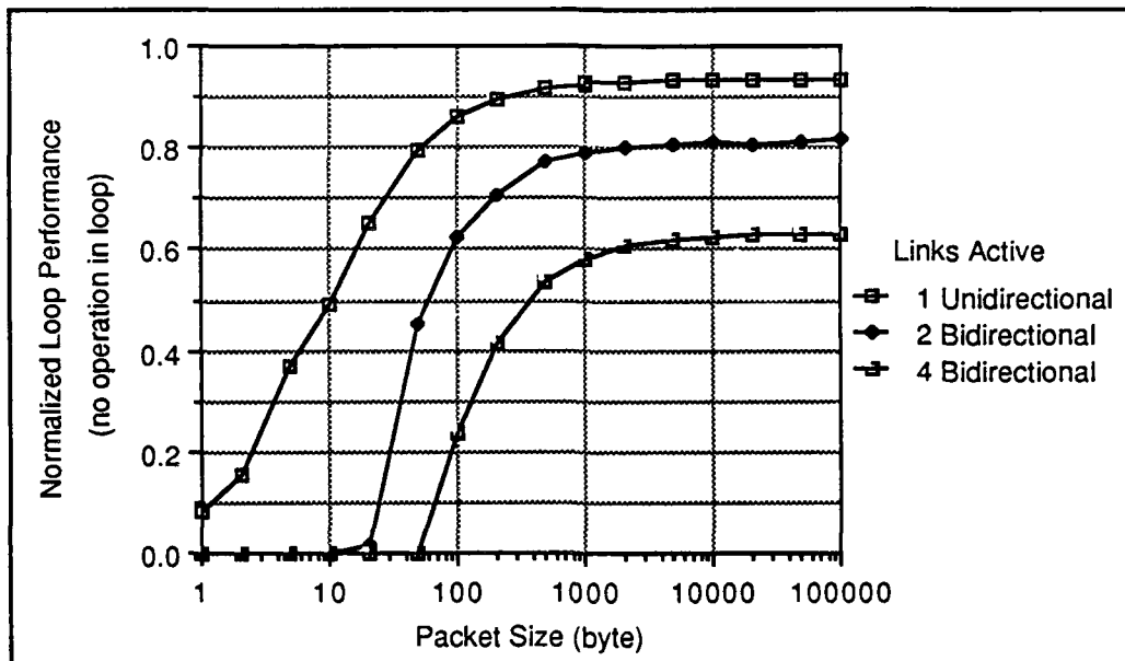
Figure 3.8. T800 Performance Degradation with No Loop Operation
