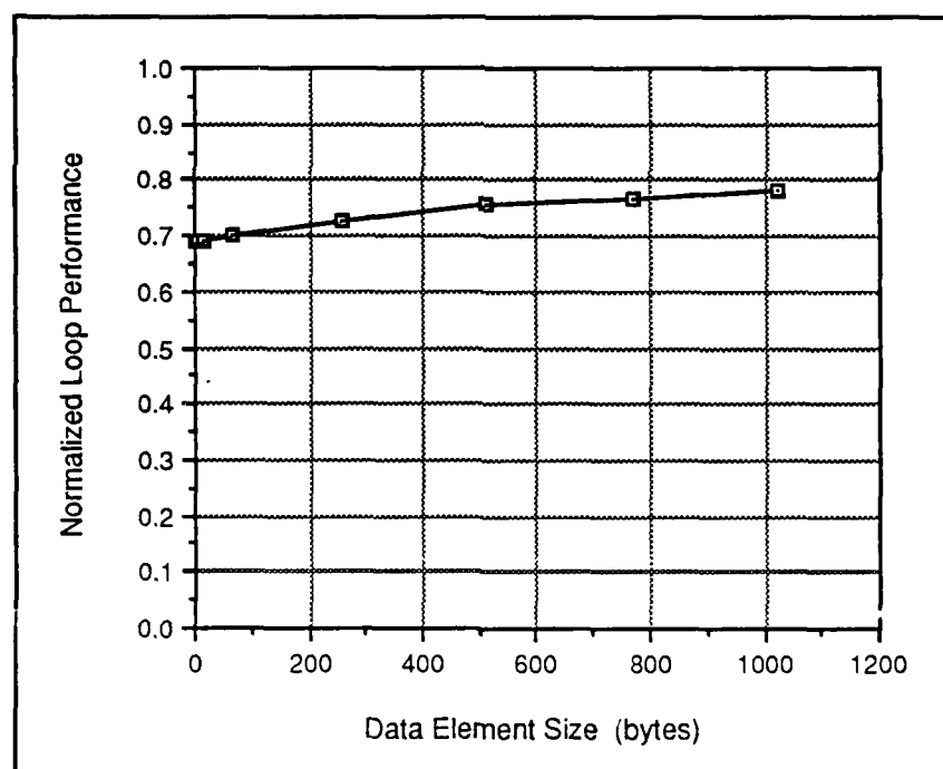
Figure 4.13. Intermediate Process Degradation During Communication
