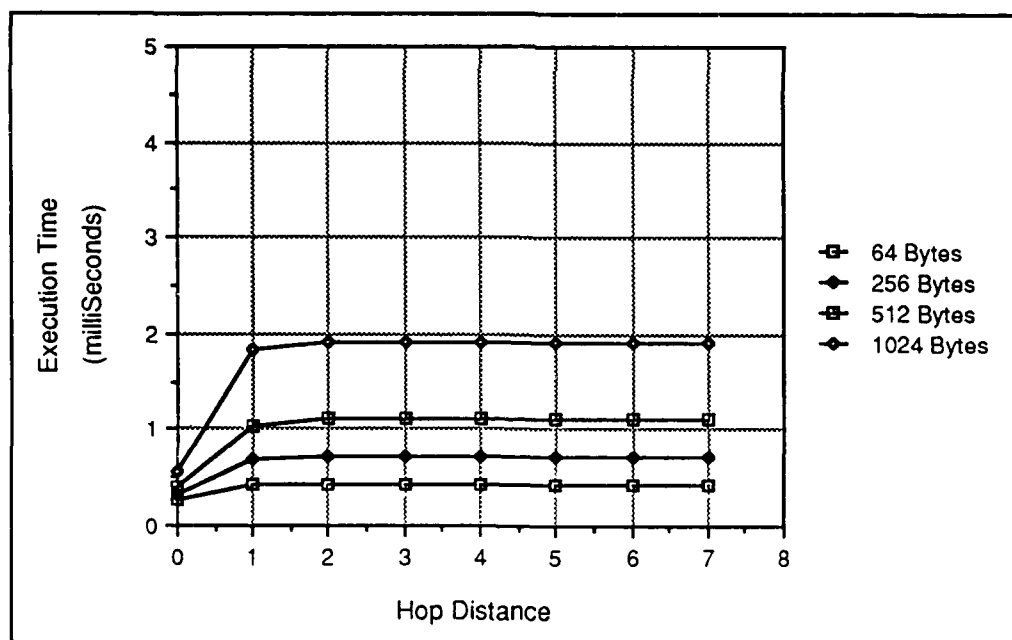
Figure 4.9. Put Operation Timing Test Results
