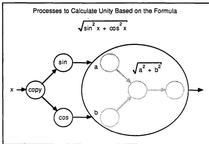
Figure 2.2. Process Abstraction Example
