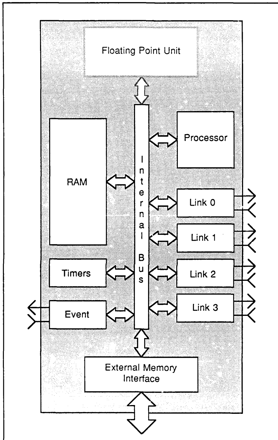
Figure 2.3. Transputer Functional Block Diagram
