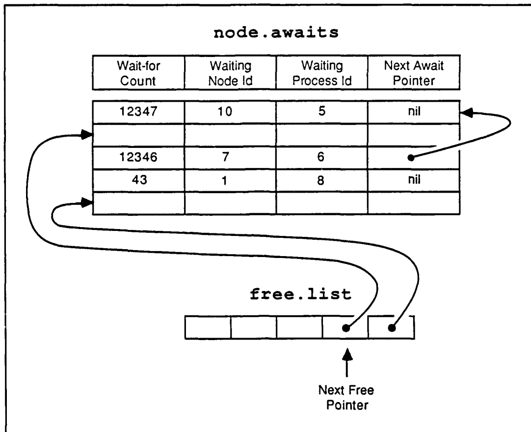
Figure 4.6. Kernel Waiting Free List Management
