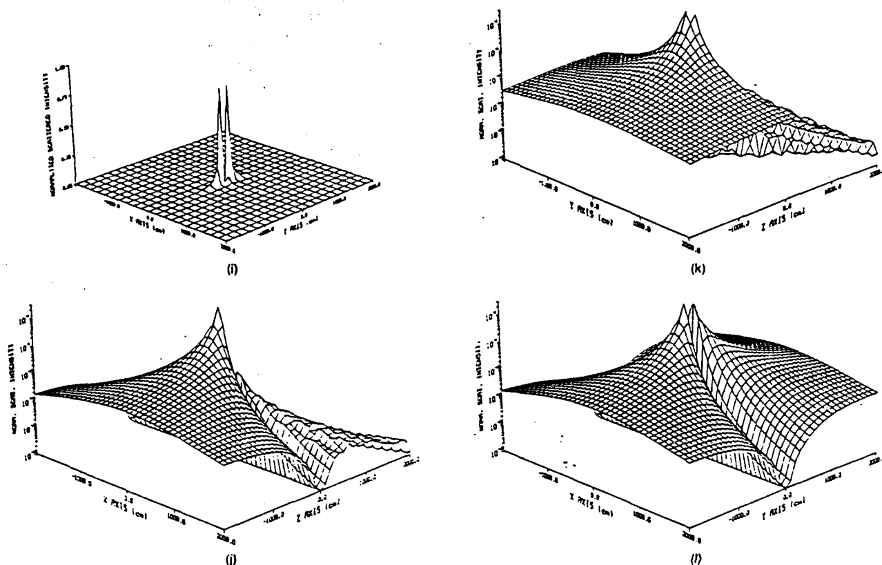
Fig. 9. Scattered far-field intensity from aluminum surfaces with R = 0.1 cm and \phi = 0 : \lambda = 1.315 \mu\text{m} in (a)–(c) and in (g)–(i); \lambda = 10.6 \mu\text{m} in (d)–(f); \lambda = 1 cm in (j)–(l). The target geometries are an ellipsoid ( \gamma = 0.5 ) in (a)–(f) and a sphere in (g)–(l).
