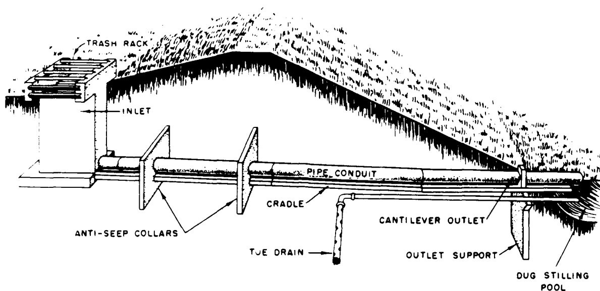
Figure 26. Drop inlet spillway. (Source: Engineering Field Manual [USDA Soil Conservation Service, Washington, DC, 1984], p 6-3.)
