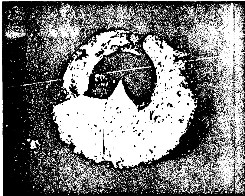
Figure 10. Fracture surface of a gas tungsten arc welded stud.
