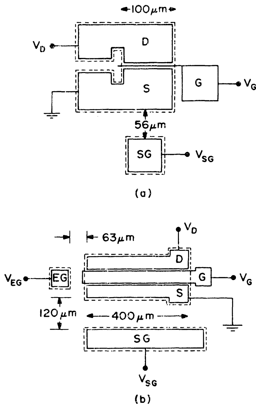
Figure 3.1 Backgating measurement configurations for (a) 2 \mu\text{m} and (b) 50 \mu\text{m} gate length MODFETs. The sidegates in (a) and (b) have dimensions 75 \mu\text{m} \times 75 \mu\text{m} and 75 \mu\text{m} \times 450 \mu\text{m} , respectively. The endgate in (b) has dimensions 75 \mu\text{m} \times 75 \mu\text{m} . Dashed line represents mesa edge.
