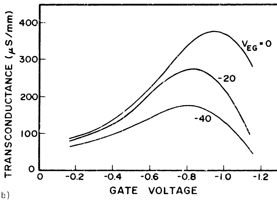
Figure 3.5 Dependence of transconductance on gate voltage as a function of endgate voltage for (a) E-mode and (b) D-mode 50 \mu\text{m} gate length MODFETs biased at V_D = 0.02 V.
