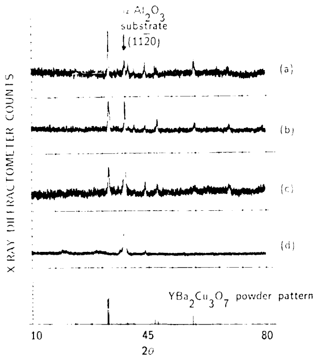
FIG. 3. X-ray data for films deposited at 400 °C on Al_2O_3 substrates. The orthorhombic phase was present after (a) 900 °C, (b) 800 °C, or (c) 700 °C anneals. As-deposited films or films annealed at (d) 600 °C were amorphous.
