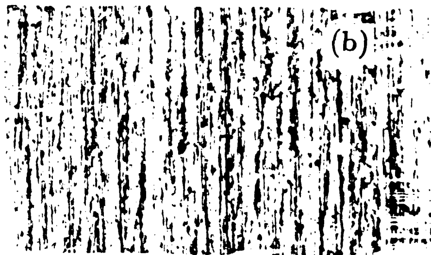
Fig. 11. Optical micrograph of steel surface preparations to 600 grade SiC paper finish followed by alkaline anodic-cleaning and acid etch, (a) 440 and (b) 1018.
