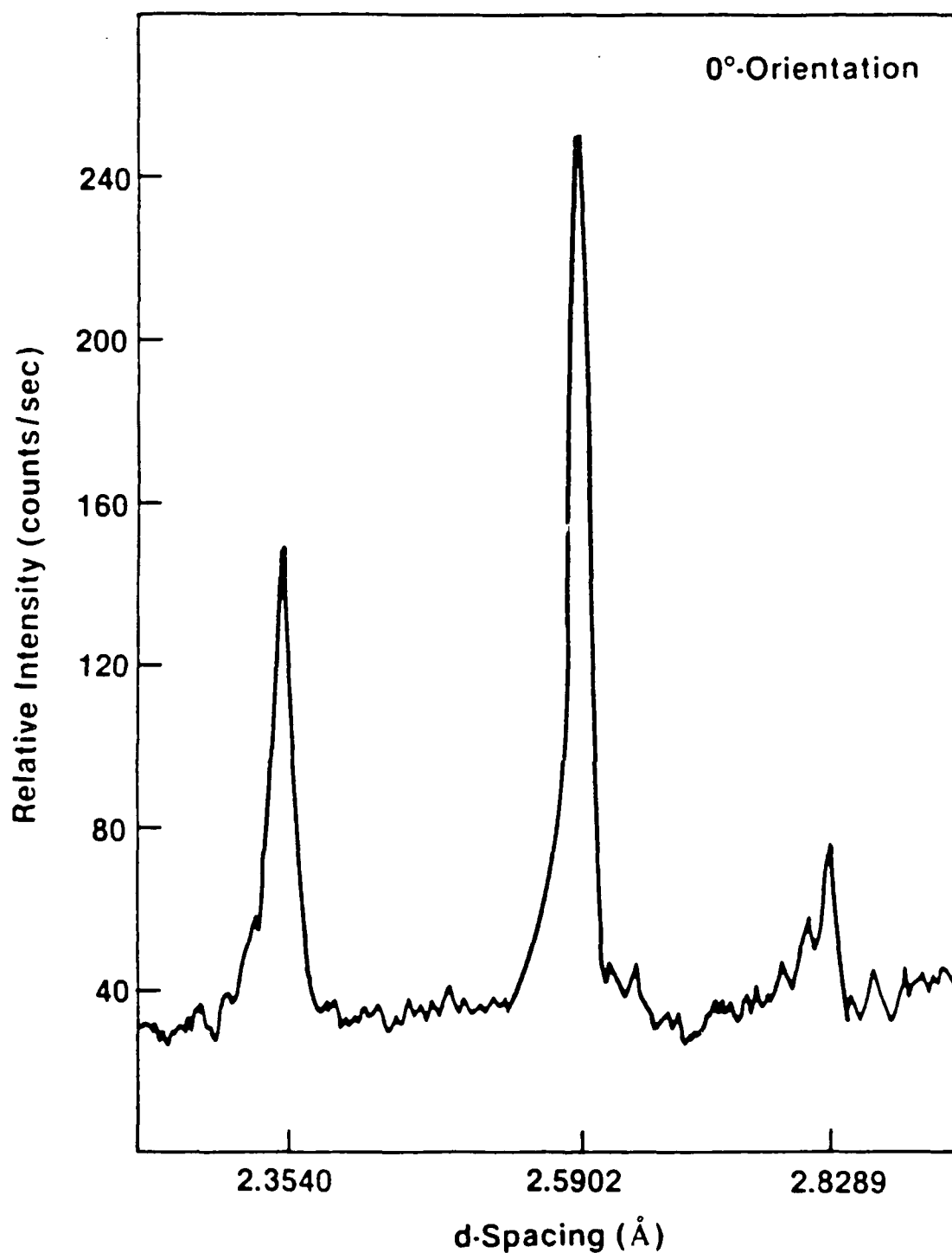
Fig. 36. X-ray diffraction pattern of cadmium electrodeposited on nickel from alkaline-cyanide electrolyte at 2 \text{ A}\cdot\text{cm}^{-2} DC (00-rotation).
