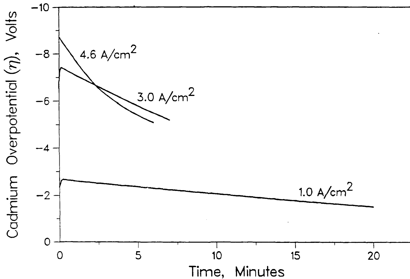
Fig. 32. Deposition potential versus \text{Cd}^{+2}/\text{Cd}^0 reference for electrodeposition of cadmium from alkaline cyanide electrolyte ( 32 \text{ g}\cdot\text{L}^{-1} \text{ Cd} , Bath B).
