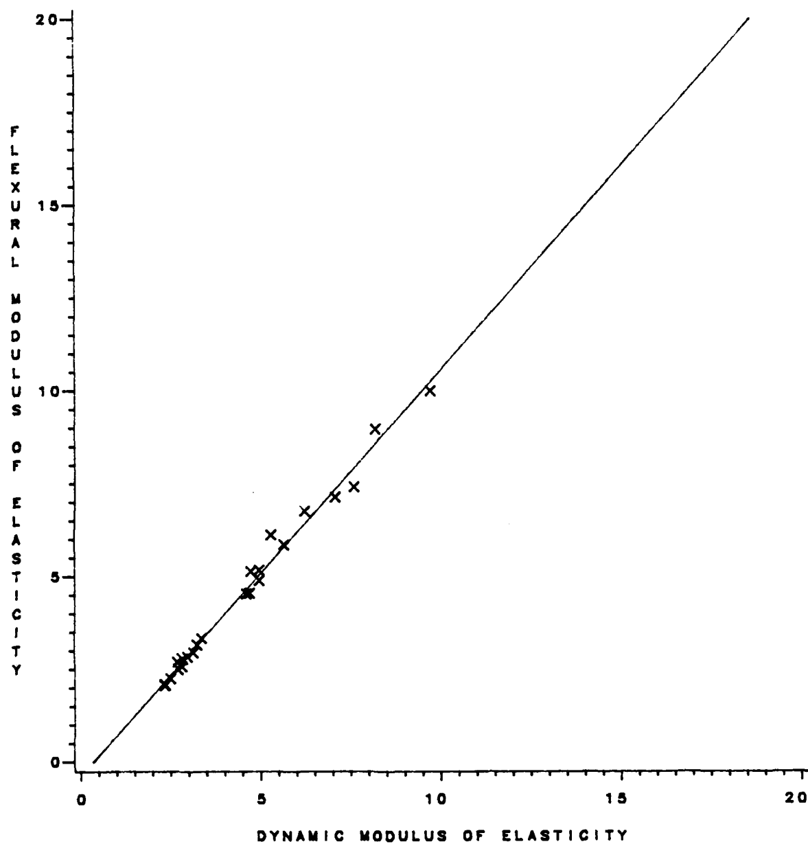
Figure 8. Scatter diagram with regression line for flexural modulus of elasticity versus dynamics modulus of elasticity - Panel 4.
