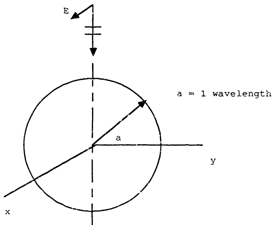
Fig 5a. Conducting sphere used as a test case for results presented in Fig. 6.
