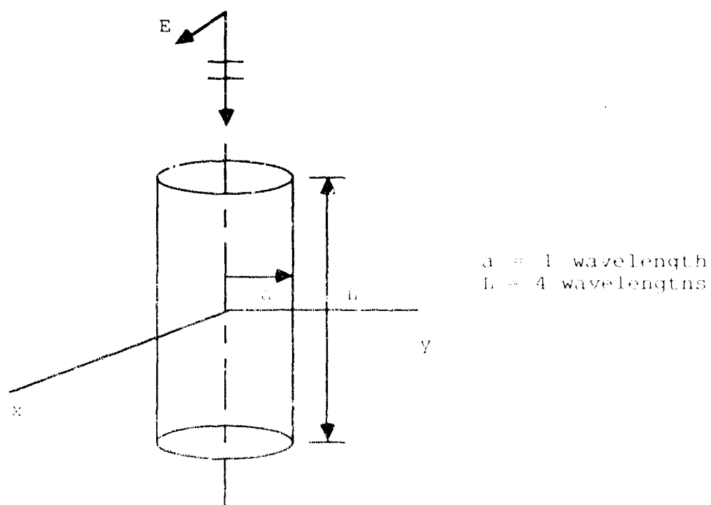
Fig. 5b. Conducting cylinder used to compute results presented in Fig. 7.
