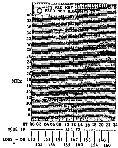
FIGURE 3a- RADAR C PREDICTION FOR WINNIPEG-RESOLUTE BAY PATH, NOV., 1959
