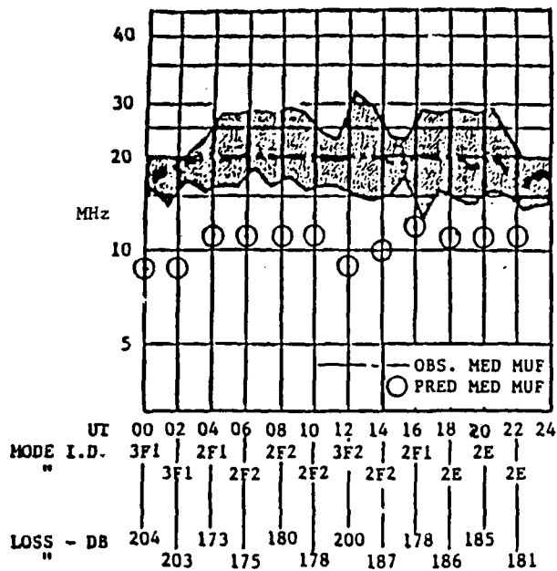
FIGURE 11a- RADAR C PREDICTION FOR ANDOYA-COLLEGE PATH, MAY, 1964
