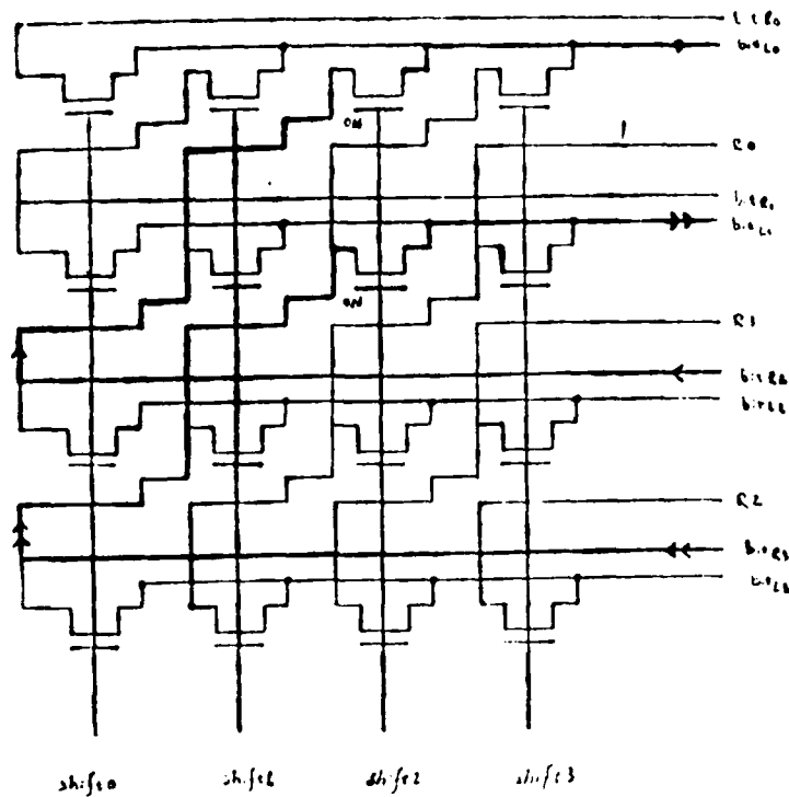
Figure 6: Barrel Shifter Schematic
