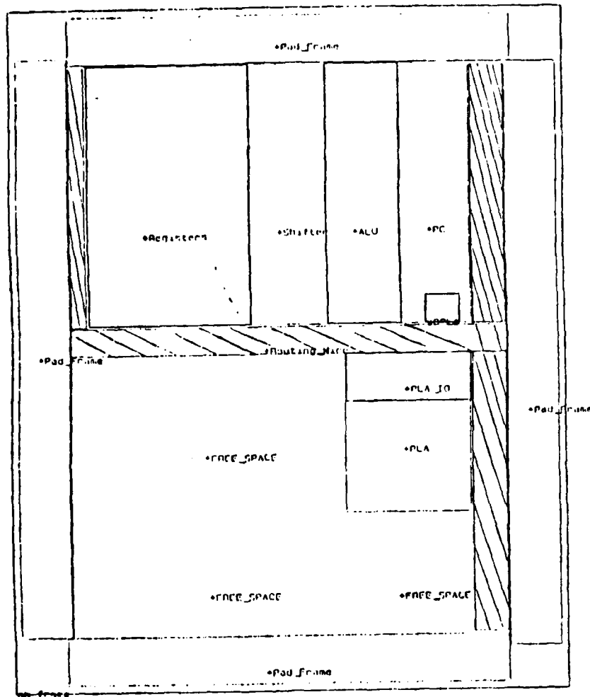
Figure 2: Floor Plan of Quarter Horse
