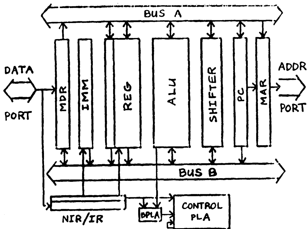
Figure 1: Datapath Schematic of Quarter Horse
