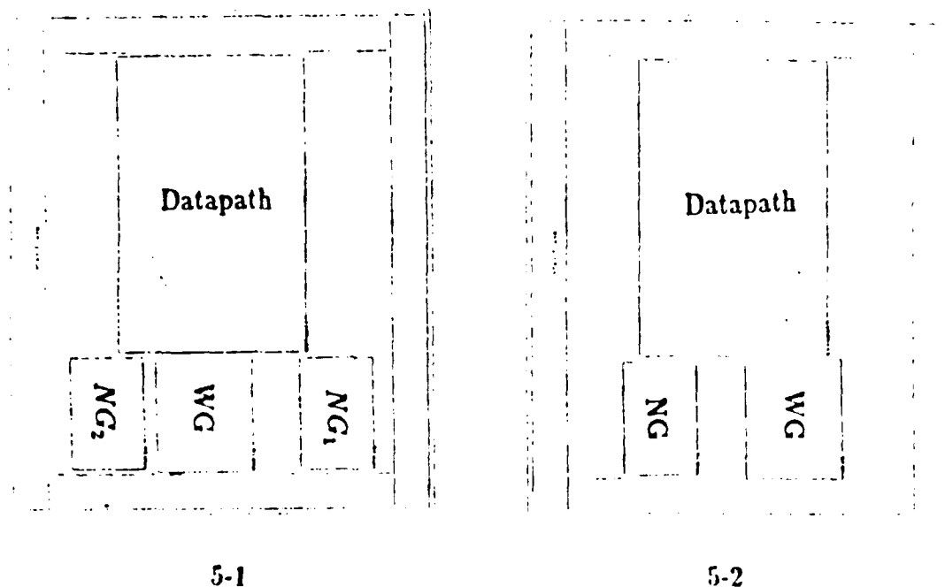
Figure 5: MIMD and SIMD floorplans
