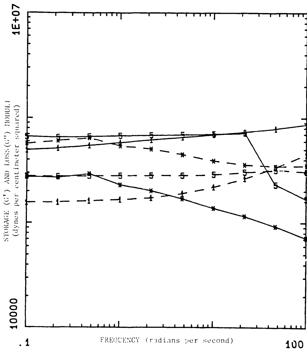
Figure 3.15. Storage and Loss Moduli vs. Frequency for PEA-PBLG Films at 5.0 Percent Strain. Wt. % PBLG: 1 (1), 5 (5), 25 (*) Modulus: G' (—), G'' (---)
