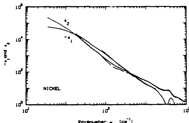
Fig. 5. Kramers-Kronig results for -\epsilon_1 and \epsilon_2 of Ni: solid line, results obtained by combining nonresonant cavity measurements with the Kramers-Kronig results obtained from our reflectance measurements (with the values of Lynch and Hunter from Ref. 1 used above 20,000 \text{cm}^{-1} ); dash-dot line for Lynch and Hunter (tabulated in Ref. 1); and dash line for the Kramers-Kronig results from averaging the reflectance in Ref. 8 with previously unpublished reflectance measurements.
