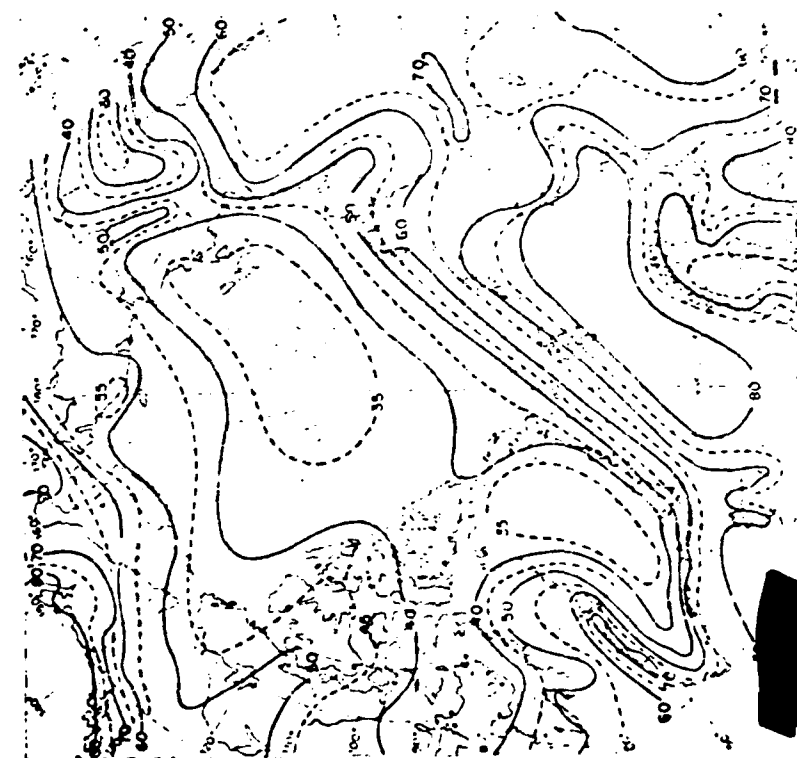
FIGURE 1-13. MEAN CLOUD COVERAGE (%) IN JANUARY
