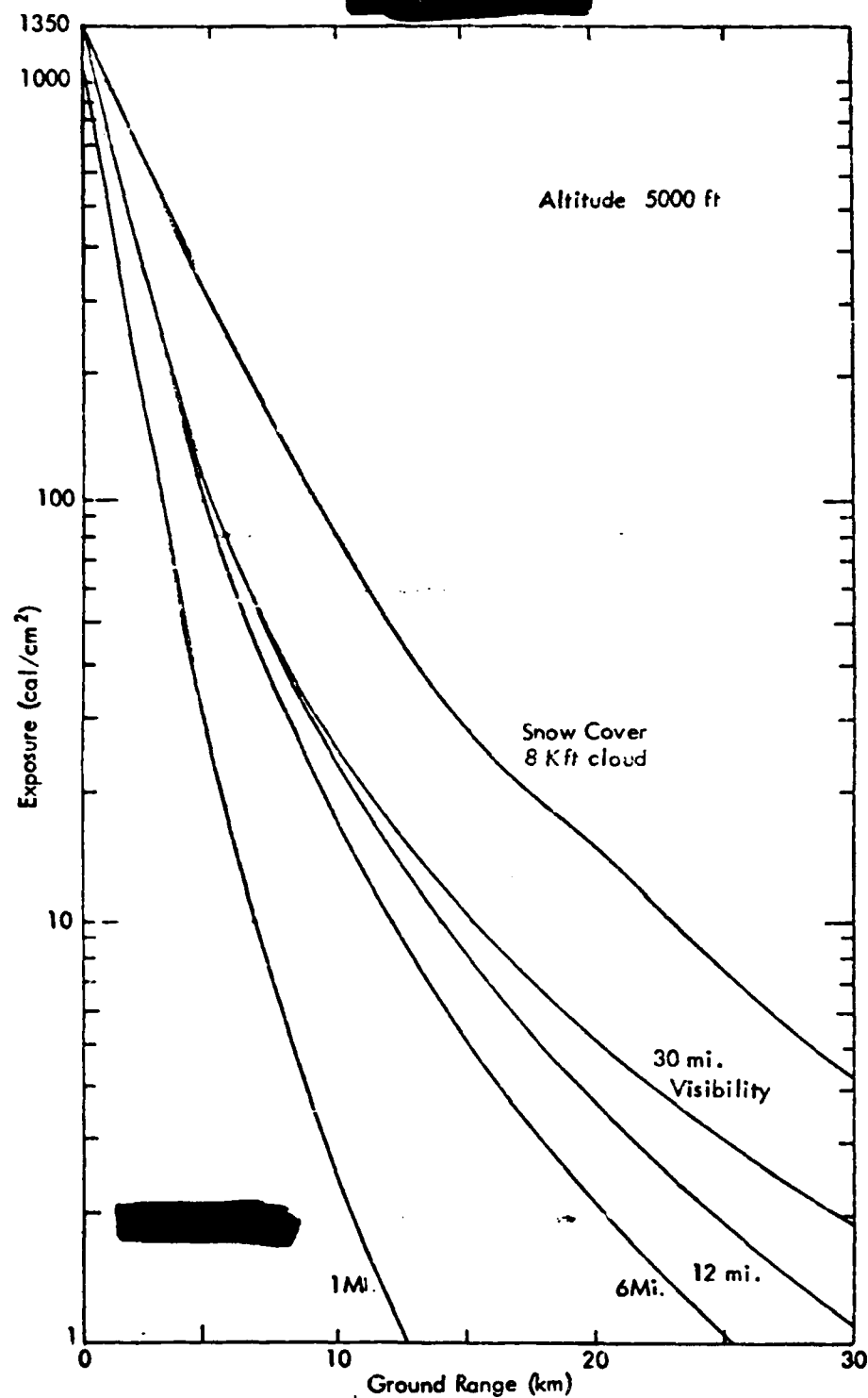
FIGURE 4-9 PREDICTED EXPOSURE VS GROUND RANGE AT SAMPLE VISIBILITIES
