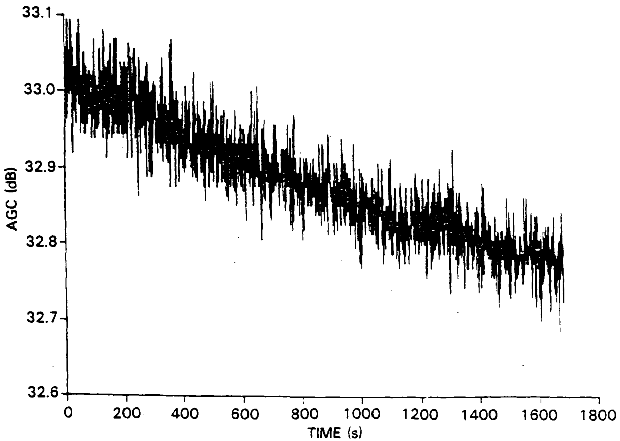
Fig. 7 — AGC record for 9-1-83 test
