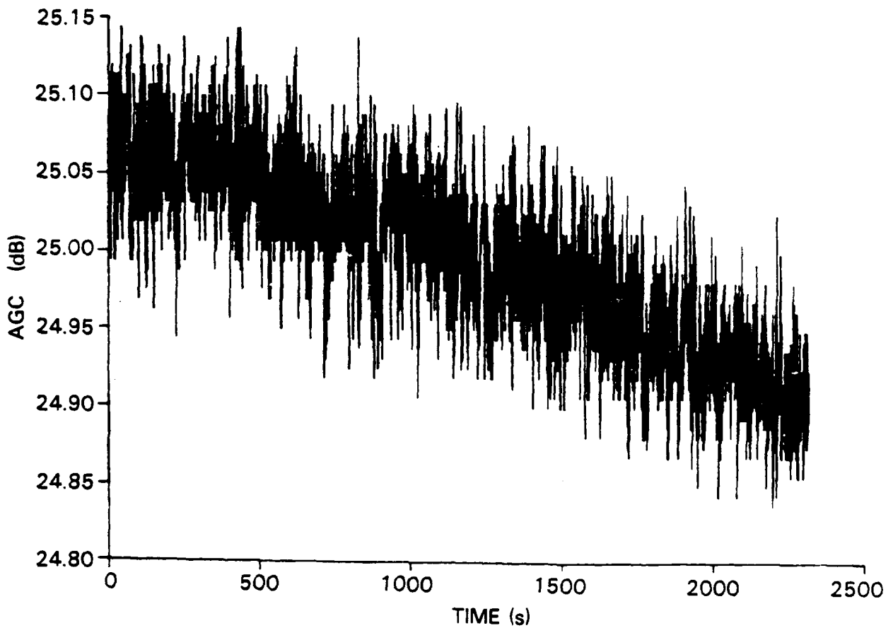
Fig. 8 — AGC record for 11-23-83
