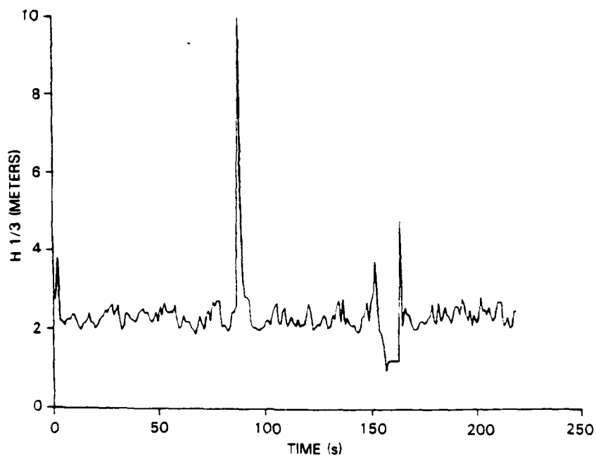
Fig. 13b — H_{1/3} response to AGC changes
