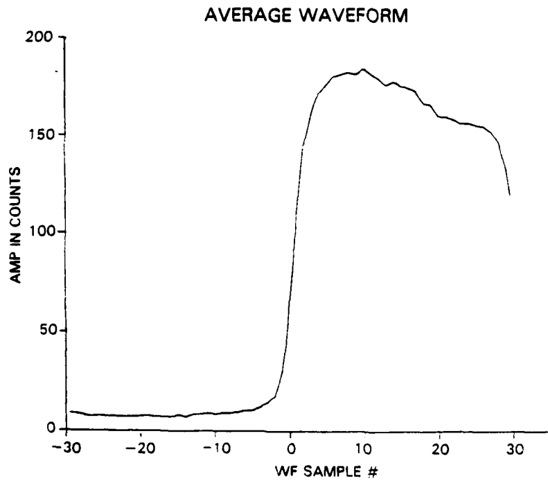
Fig. 14b — 36 second average waveform from 11-23-83 test, segment 1A,2B
