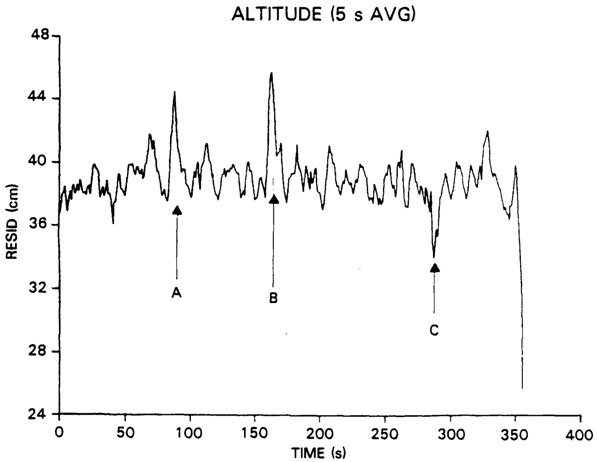
Fig. 9a — Altitude disturbances (A,B,C) correlated with AGC transients (A,B,C) for 11-23-83 data
