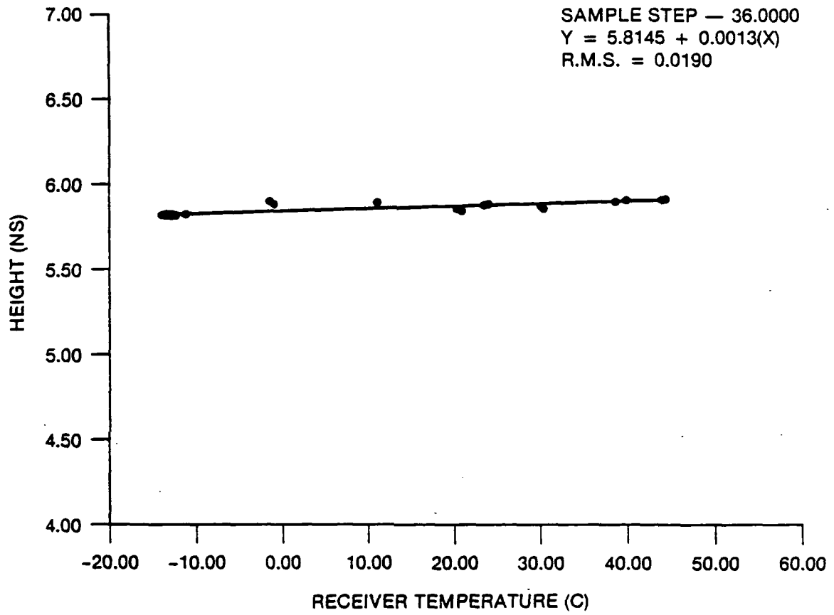
Fig. B4 — Calibration mode height as a function of receiver temperature
