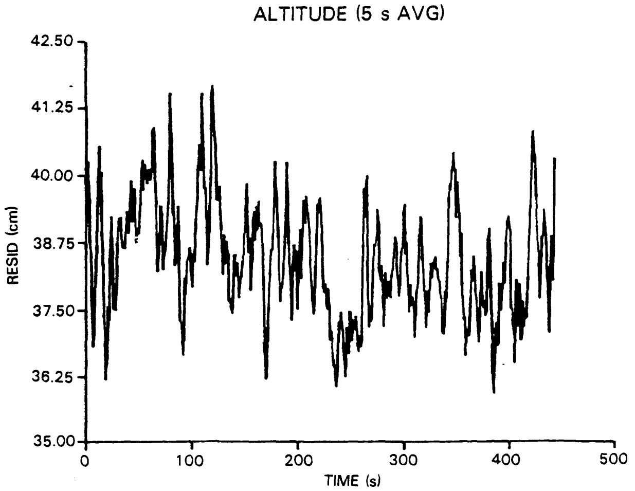
Fig. 11a — Altitude response to changes in AGC for 11-23-83
