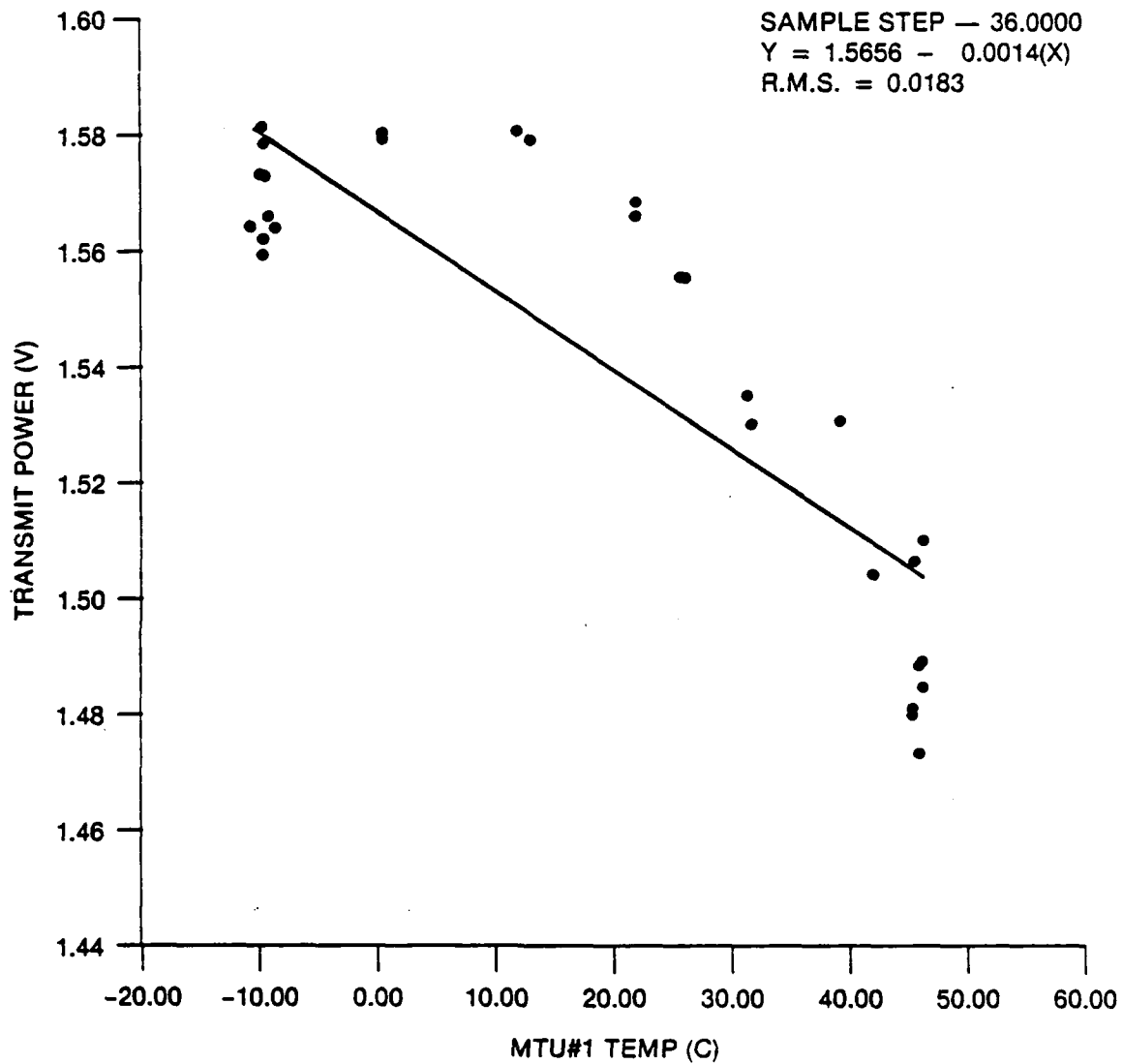
Fig. B6 — Transmit power as a function of MTU temperature
