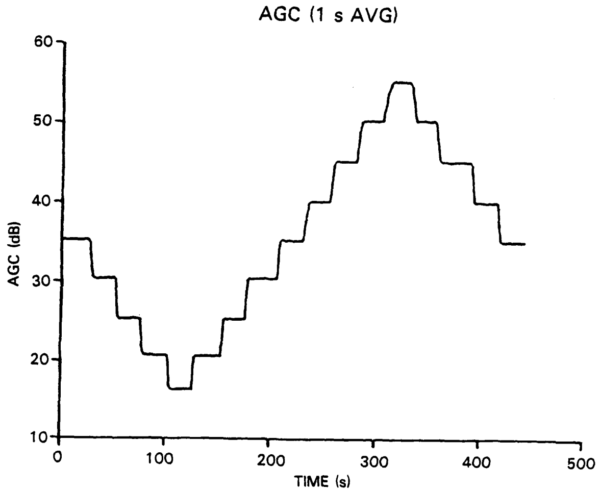
Fig. 11b — Altitude response to changes in AGC for 11-23-83
