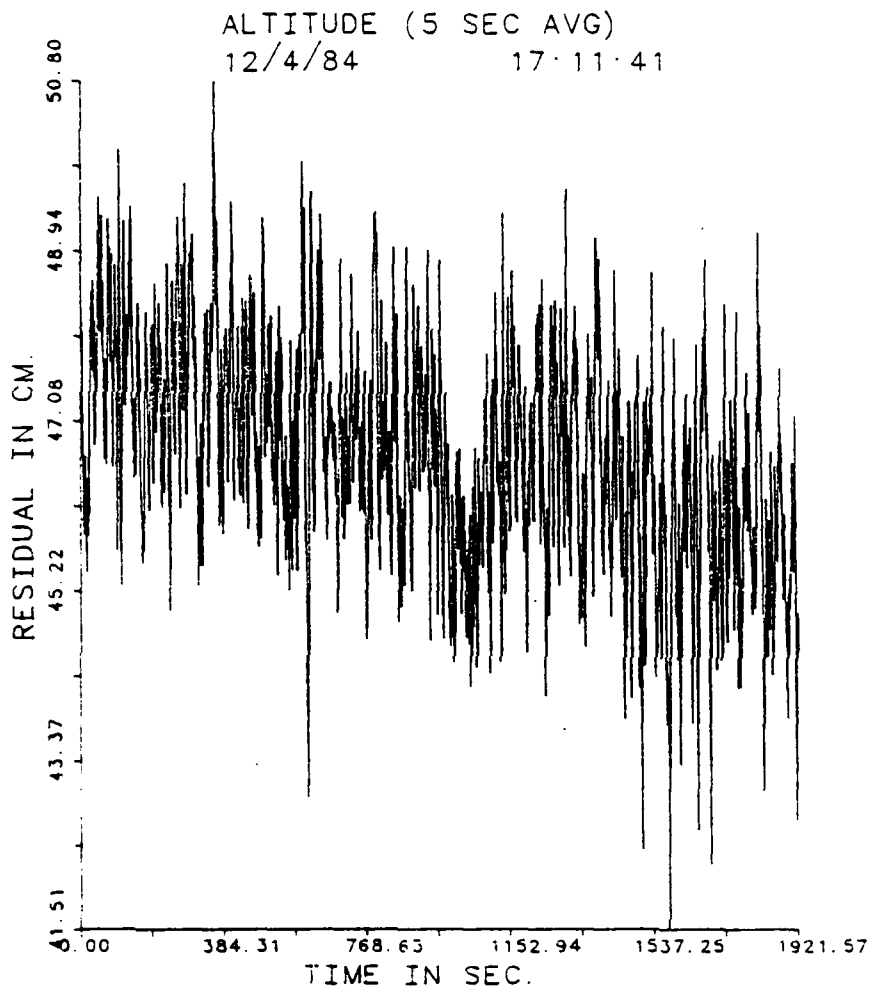
Fig. 4b — Five-second averaged height data — 12-4-84 test
