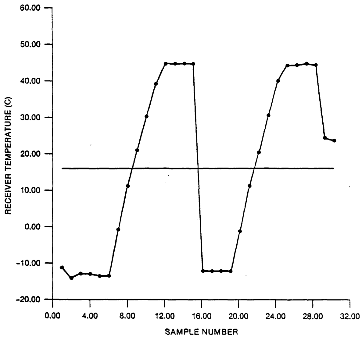
Fig. B3 — Receiver temperature profile
