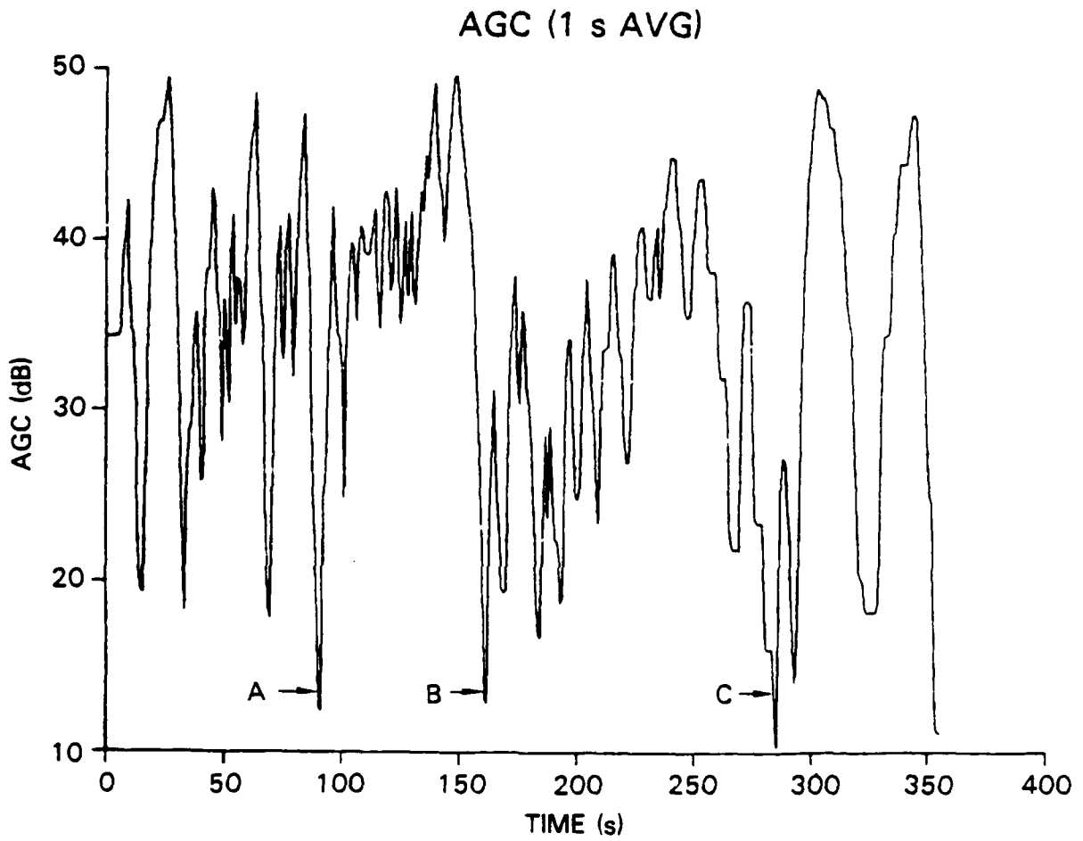
Fig. 9b — Altitude disturbances (A,B,C) correlated with AGC transients (A,B,C) for 11-23-83 data
