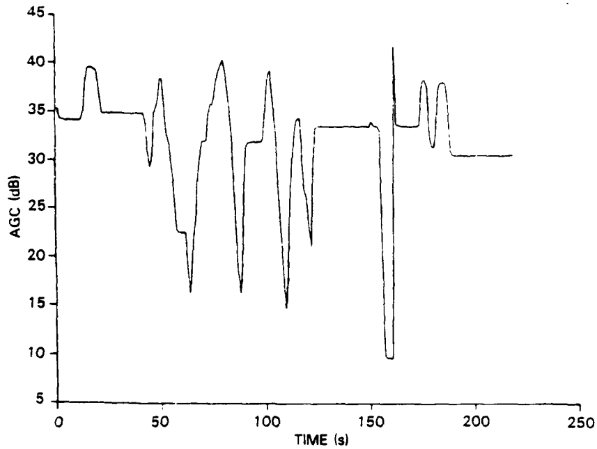
Fig. 13a — Manually inserted AGC changes made during test
