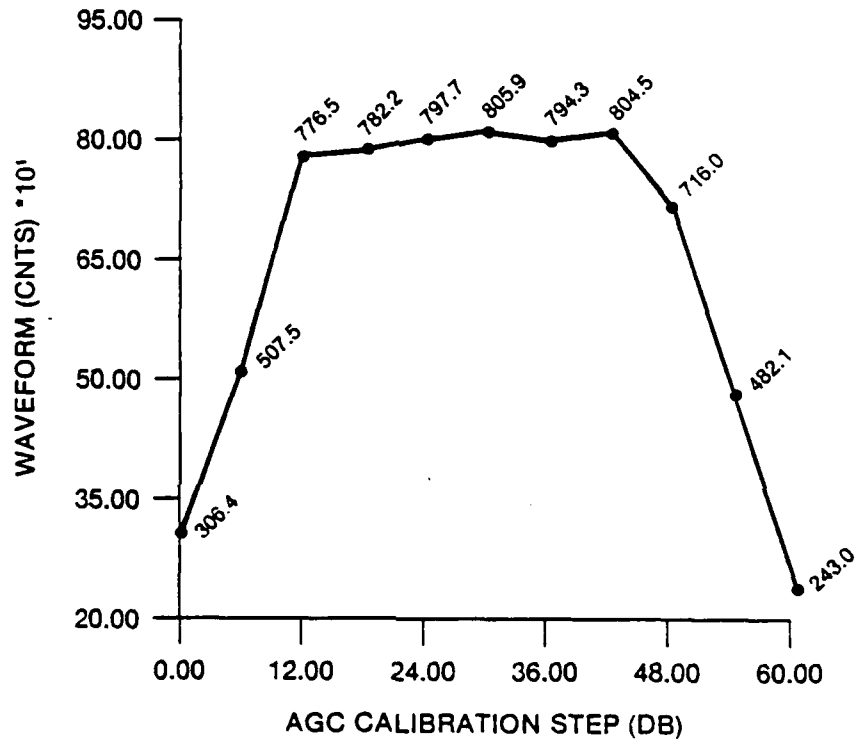
Fig. B1 — Waveform sample 0 for each calibration step
