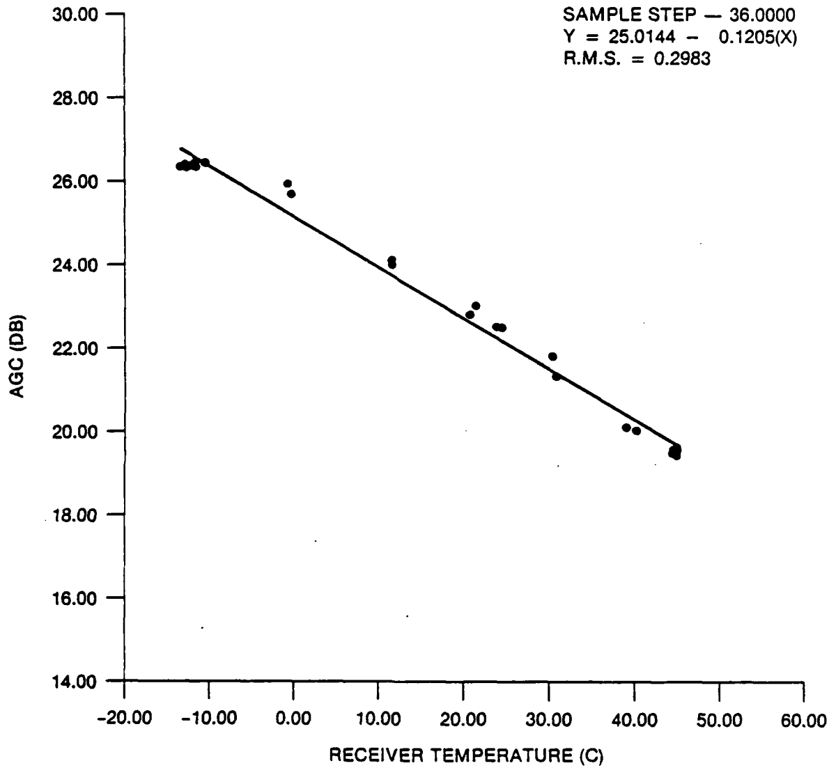
Fig. B5 — AGC as a function of receiver temperature
