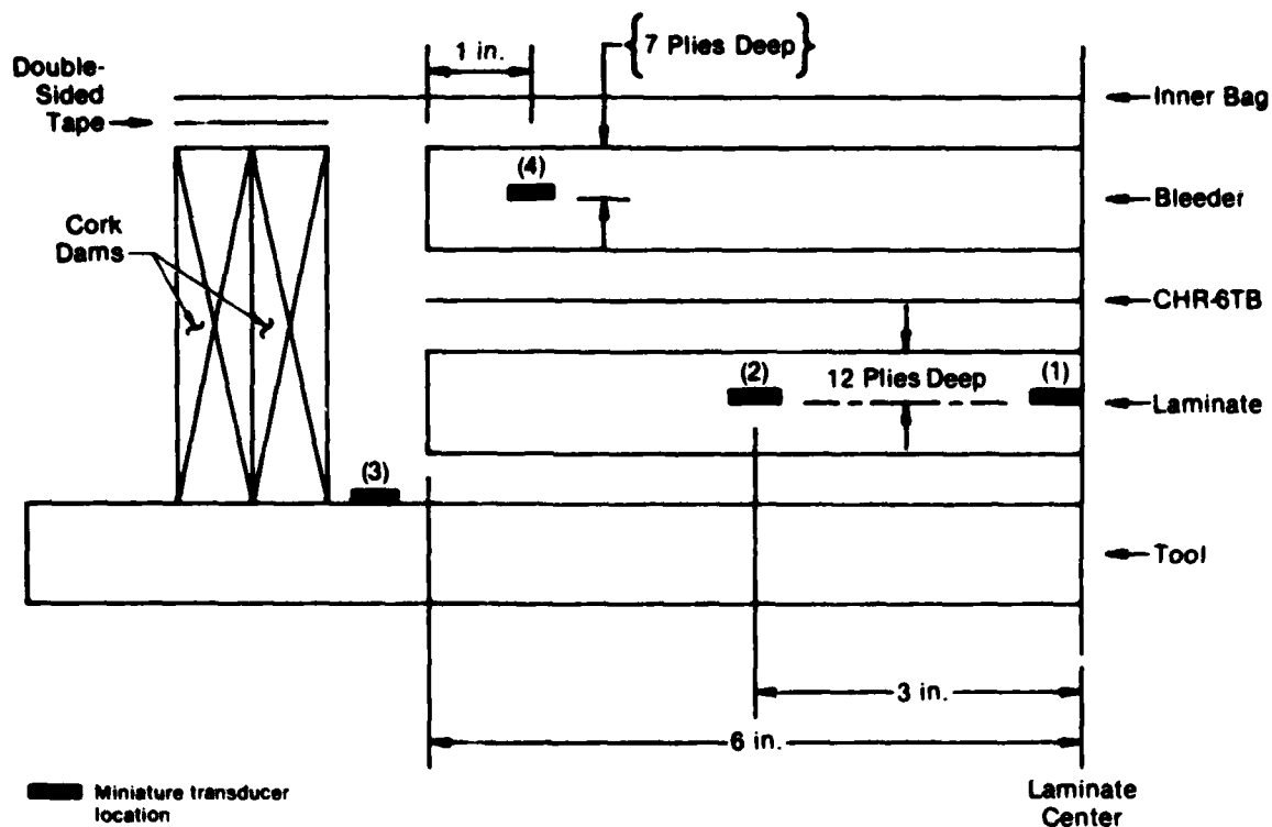
Figure 65. Miniature Transducer Location for Horizontal Flow Laminates
