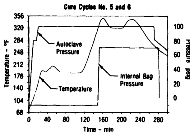
Figure 87. Sensor Demonstration Laminate Cure Cycles
