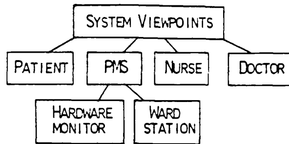
FIGURE 3.3.1-5 FIRST SOLUTION - REFINEMENT OF PMS VIEWPOINT.
