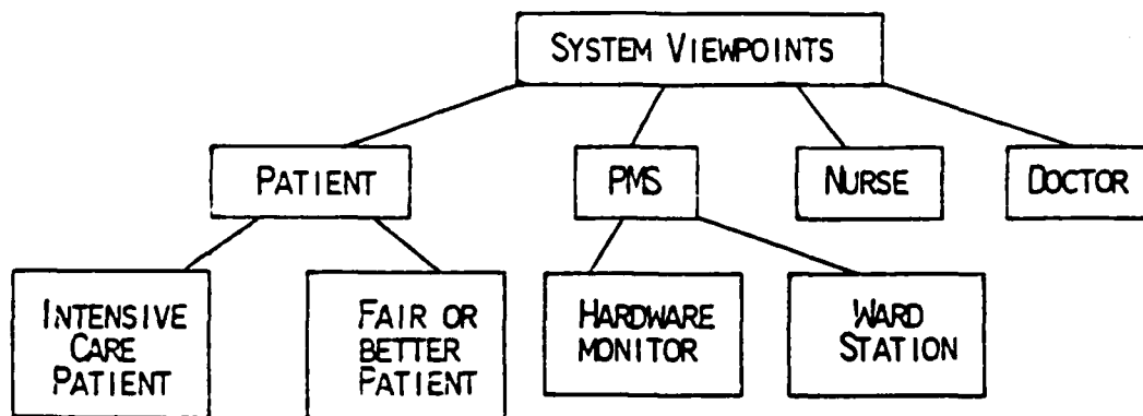
FIGURE 3.3.1-7 REVISED SOLUTION - REFINEMENT OF PMS VIEWPOINTS.
