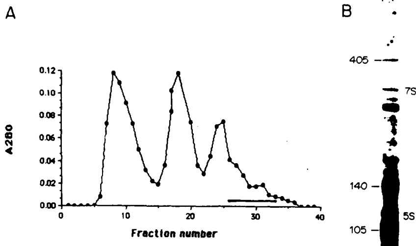
Figure 5. Fractionation of RNaseP activity by gel filtration. A. Gel filtration of a 6-10a PEG precipitate from a H. volcanii S30 extract on Sepharose 4B. Active fractions are indicated by the solid bar. B. pCp end labeling of RNAs from fraction 31. RNAs which copurify with RNaseP activity are indicated.
