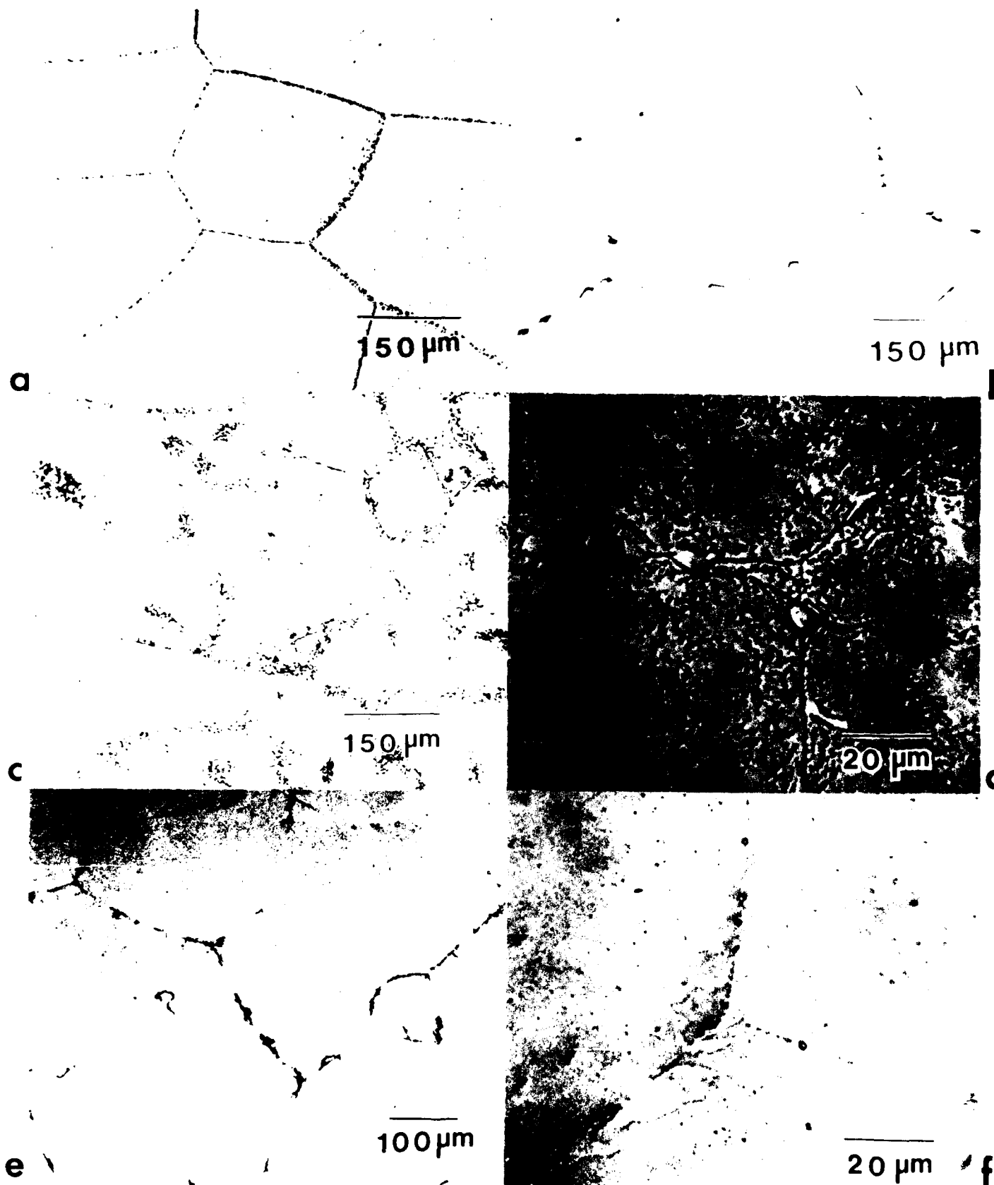
Figure 21 Optical micrographs of the 30Nb alloy, solution annealed at 1250^{\circ}\text{C} ( 2282^{\circ}\text{F} ) for 4h, water quenched, re-aged at the temperatures listed below and water quenched (a) 1250^{\circ}\text{C} ( 2282^{\circ}\text{F} ), 4h; (b) 1200^{\circ}\text{C} ( 2192^{\circ}\text{F} ), 4h; (c) 1100^{\circ}\text{C} ( 2012^{\circ}\text{F} ), 4h; (d) 1000^{\circ}\text{C} ( 1832^{\circ}\text{F} ), 4h; (e) 900^{\circ}\text{C} ( 1652^{\circ}\text{F} ), 24h; (f) 800^{\circ}\text{C} ( 1472^{\circ}\text{F} ), 24h.
