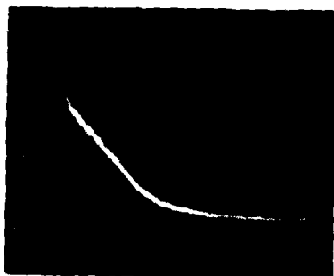
Fig. 6. The decay behavior of the thermal grating of a "dye" PCH sample when the grating maxima give rise to liquid phase. Time scale is 50 ms/div. The observed relaxation time of \sim 150 ms is consistent with the theoretical prediction based on reorientation mechanisms.
