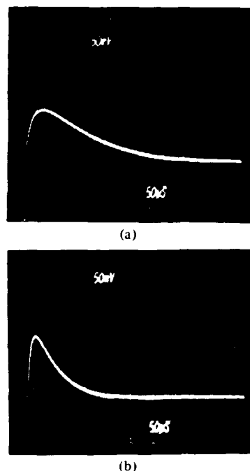
Fig. 5. (a) The decay of the thermal grating as monitored by the He-Ne diffraction. Time scale is 50 \mu\text{s}/dw . The grating wave vector \vec{q} is perpendicular to the director axis \vec{n} . (b) Thermal grating decay for \vec{q} parallel to the director axis \vec{n} . Decay is shorter by a factor of two.
