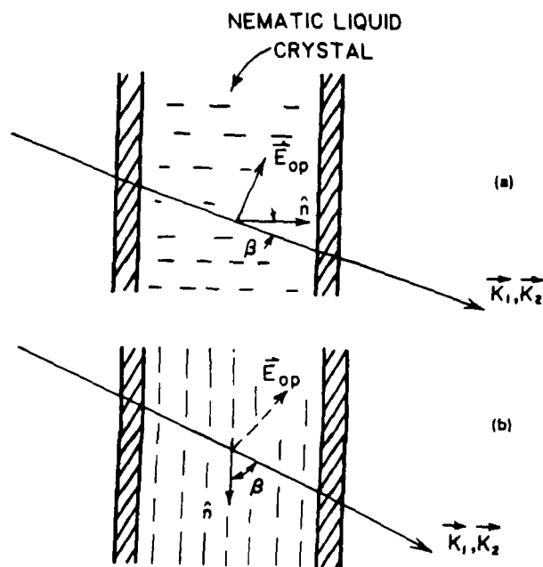
Fig. 2. Schematics of laser propagation in (a) a homeotropic nematic liquid crystal film and (b) a planar nematic film. \mathbf{K}_1 and \mathbf{K}_2 are the propagation wave vectors; \mathbf{E}_{op} is the optical field vector. The two laser beams lie in a plane perpendicular to the paper and intersect at a wave-mixing angle on the film.
