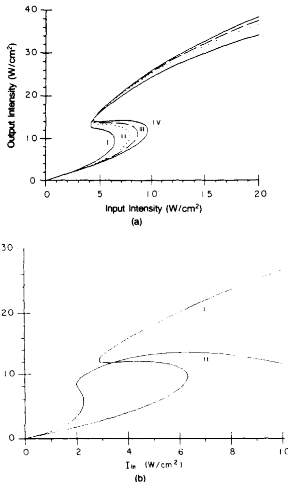
Fig. 7. (a) Transverse optical bistability for the case \beta = 22^\circ , showing how the switching changes as the width of the reorientation profile is varied. Curve I: width of \theta(r) = laser width, i.e., local response; curve II: width of \theta(r) = 1.5-laser width; curve III: width of \theta(r) = 2-laser width; curve IV: width of \theta(r) = 4-laser width. (b) Transverse optical bistability for the case \beta = 0^\circ . Curve I: local response, width of \theta(r) = laser width; curve II: width of \theta(r) = 1/3 laser width showing markedly different switching characteristics.
