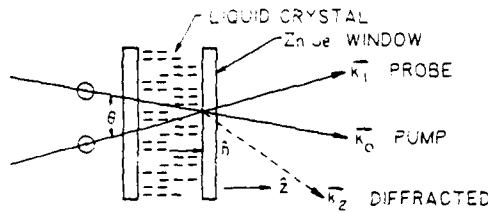
Fig. 1. Schematic of the amplification of a weak probe beam ( E_1 , k_1 ) by a strong pump beam ( E_0 , k_0 ) and the simultaneous generation of the principal diffracted beam ( E_2 ). The laser is polarized in a direction perpendicular to the plane of the paper.
