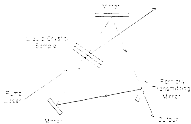
Fig. 6 One of several possible ring oscillators that can be constructed using the beam amplification effect.
