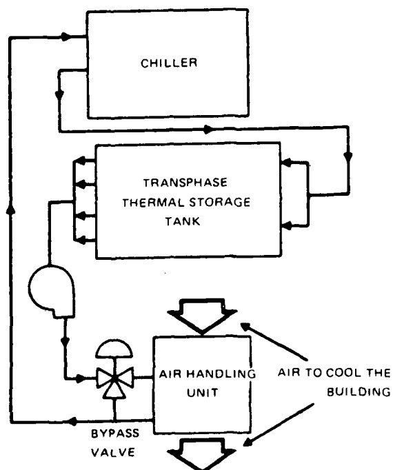
Figure 10. Typical layout of a eutectic salt system.
