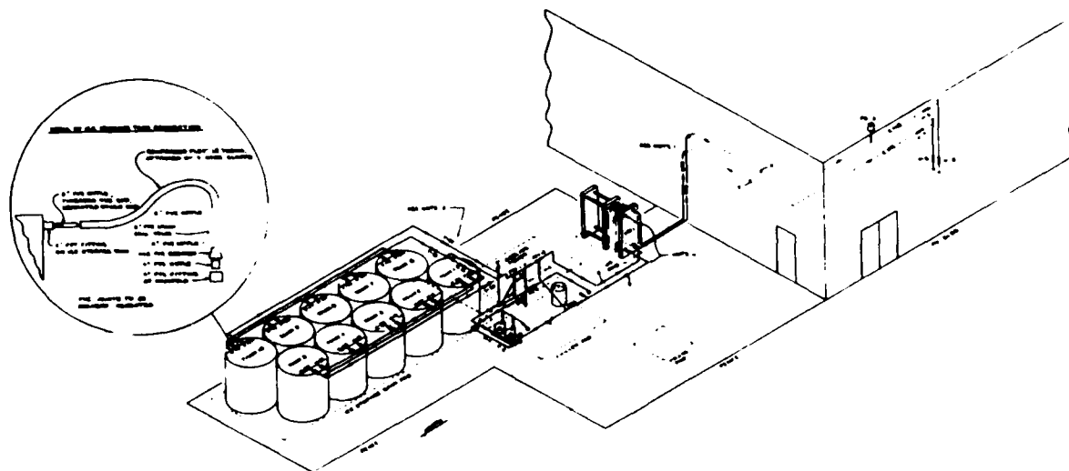
Figure 23. Ice system isometric.
