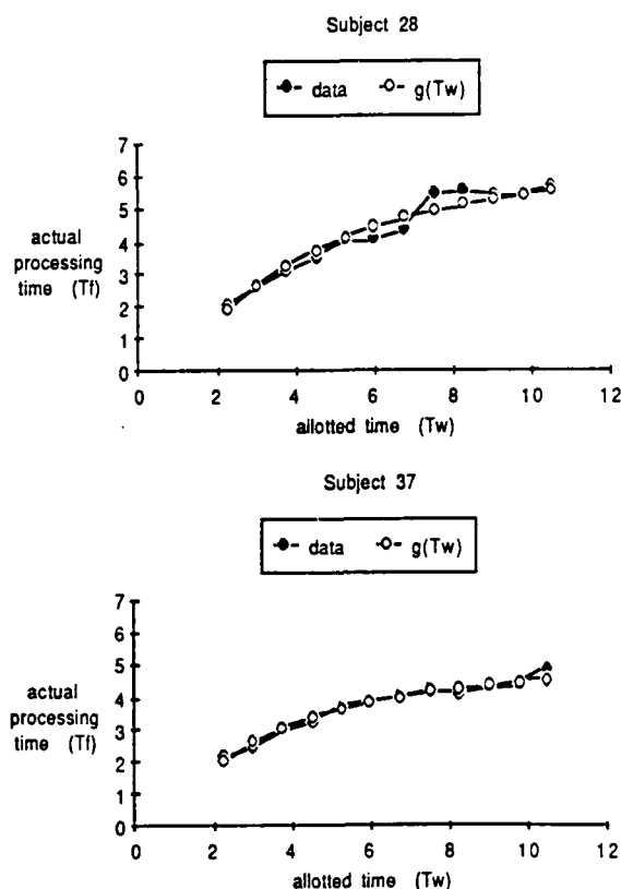
Fig. 2 Exponential Fit for Two Subjects
