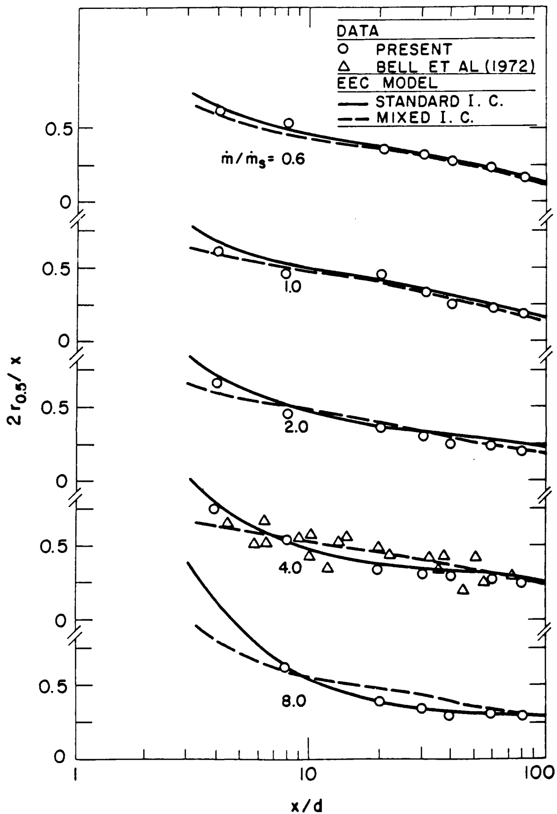
Figure 18. Streamwise variation of characteristic void-fraction diameter for round jets.
