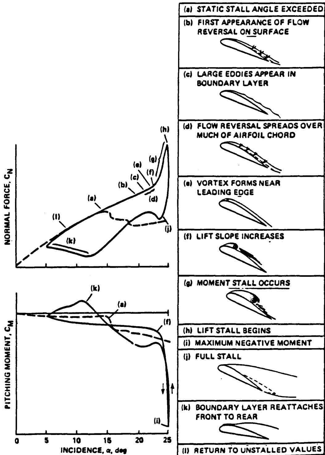
Figure 1. Dynamic Stall
