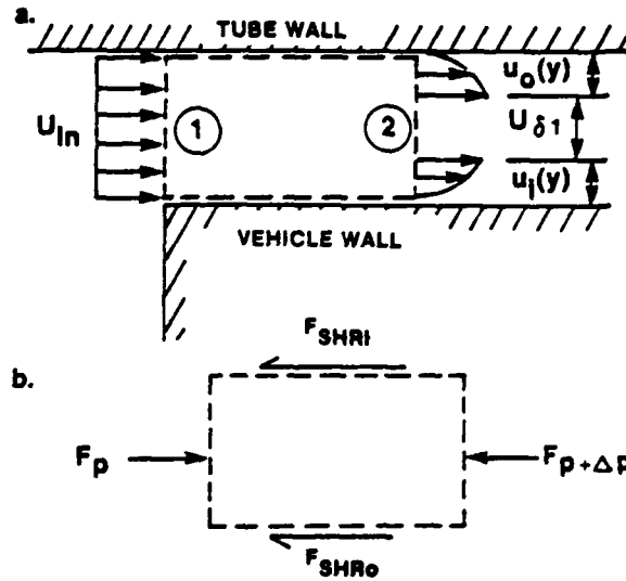
Figure 3-9. Control Volume of Annular Gap
