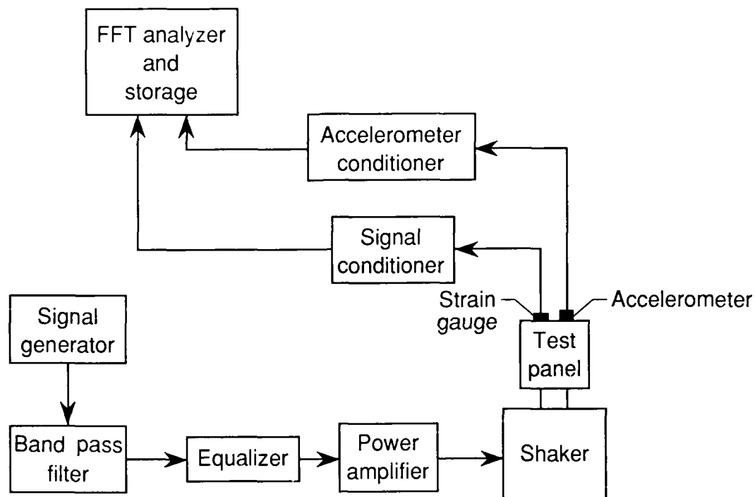
Figure 4. Diagram of instrumentation setup.
