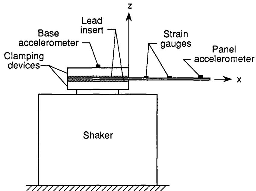
(a) Cantilevered apparatus.
