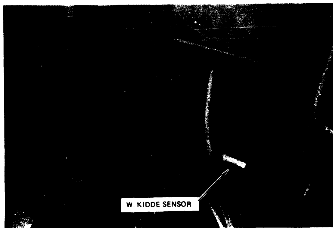
Figure 11. W. Kidde Sensor Units Installed in AENFTS on Forward Bulkhead
