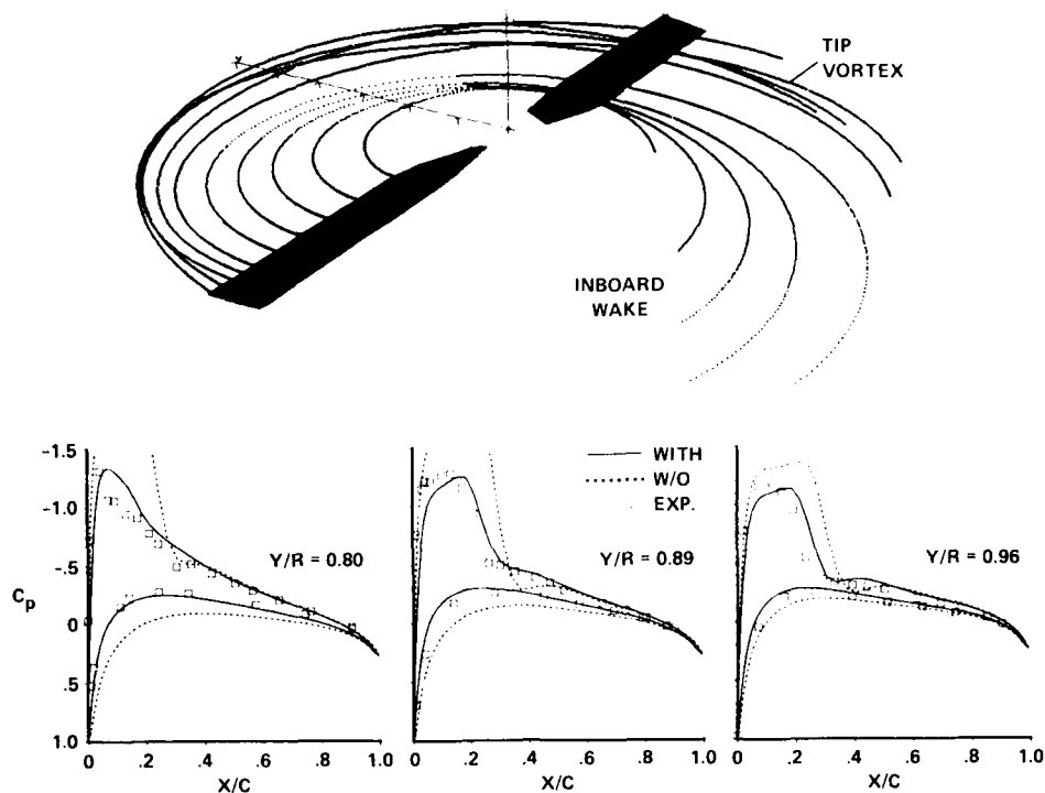
Figure 14. Streamlines and pressure distributions on a two-blade rotor in hover; Euler solution, M_T = 0.794 , \theta = 8^\circ , AR = 6
