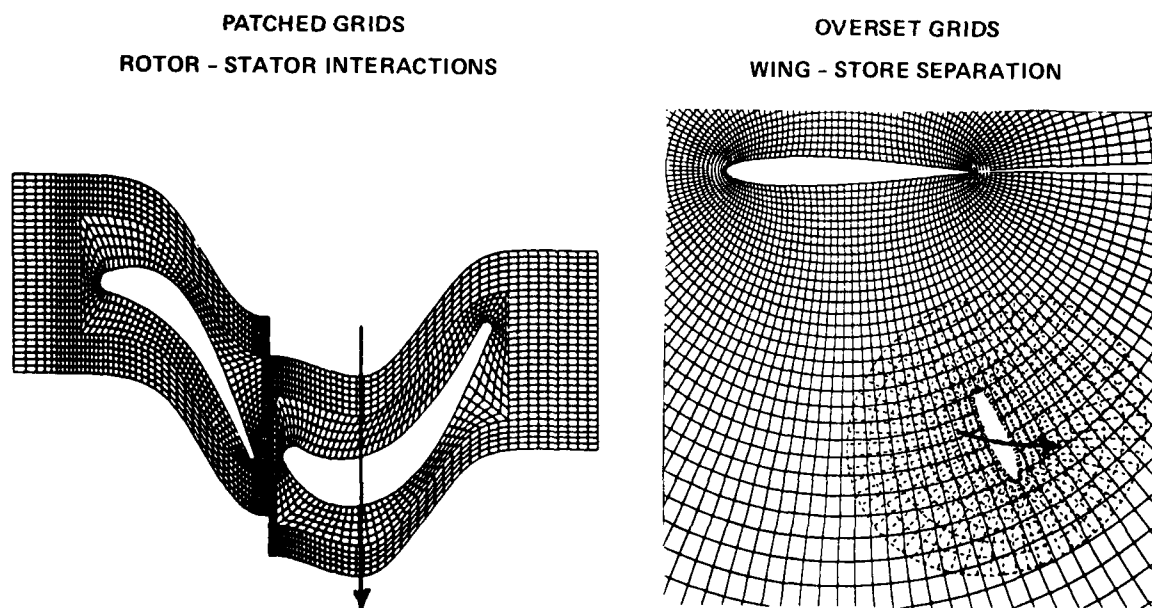
Figure 17. Example of grid interfaces in relative motion
