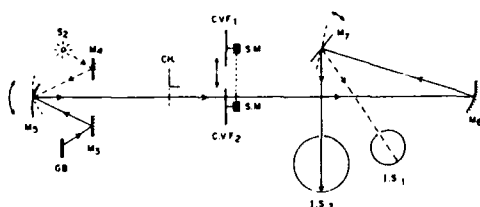
Fig. 2. Optical system for measurements in the infrared region (schematic): S_2 , projector lamp; M_3, M_4, M_5 , plane mirrors; M_6, M_6 , spherical mirrors; GB , globar; IS_1 , integrating sphere for the FIR region; IS_2 , integrating sphere for the NIR region; CVF_1, CVF_2 , circular variable filters.
