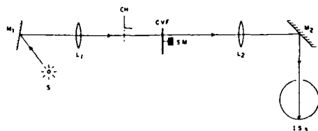
Fig. 1. Optical system for reflectance measurements in the VIS region: S , source; M_1, M_2 , plane mirrors; L_1, L_2 , lenses; IS_1 , integrating sphere; CVF , circular variable filter.
