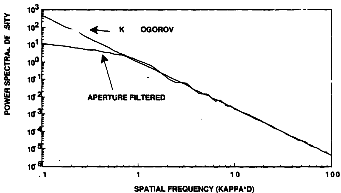
Figure 3-24. Unfiltered and aperture filtered Kolmogorov turbulence spectrums.
