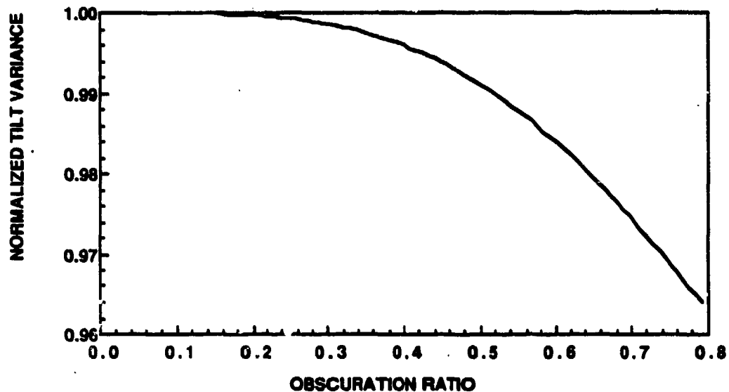
Figure 3-19. Normalized Zernike tilt for an annular aperture.
