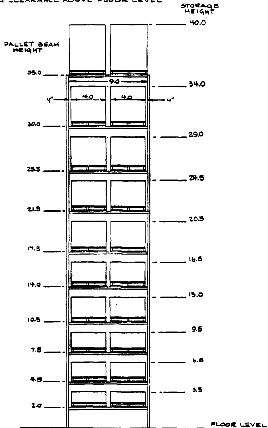
FIGURE 5 CAPS PALLET RACK ELEVATION
