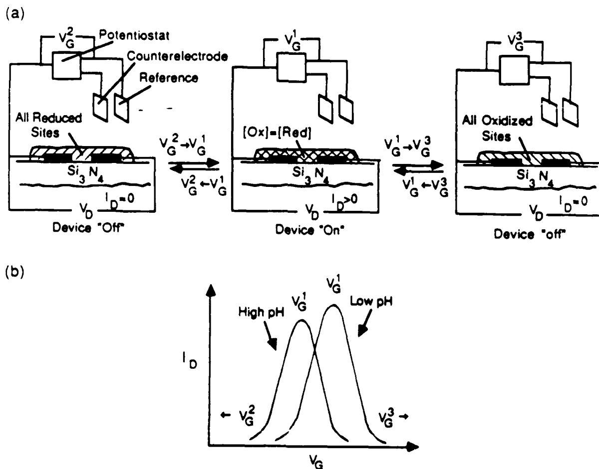
Scheme 1. (a) A microelectrochemical transistor based on a conventional redox polymer operated at a small value of V_D . The device is only turned on to a significant extent at V_G = E^\circ , V_G^1 . At V_G significantly ( >0.2 V) more negative ( V_G = V_G^2 ) or positive ( V_G = V_G^3 ) of E^\circ only the reduced or oxidized sites are present, respectively, and the device is off. (b) The I_D - V_G characteristic of a microelectrochemical transistor based on a redox polymer such as
