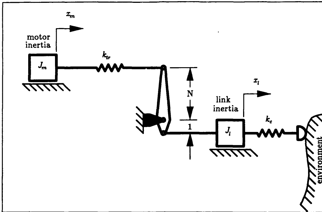
Figure 4.8. Transmission model for force control.
