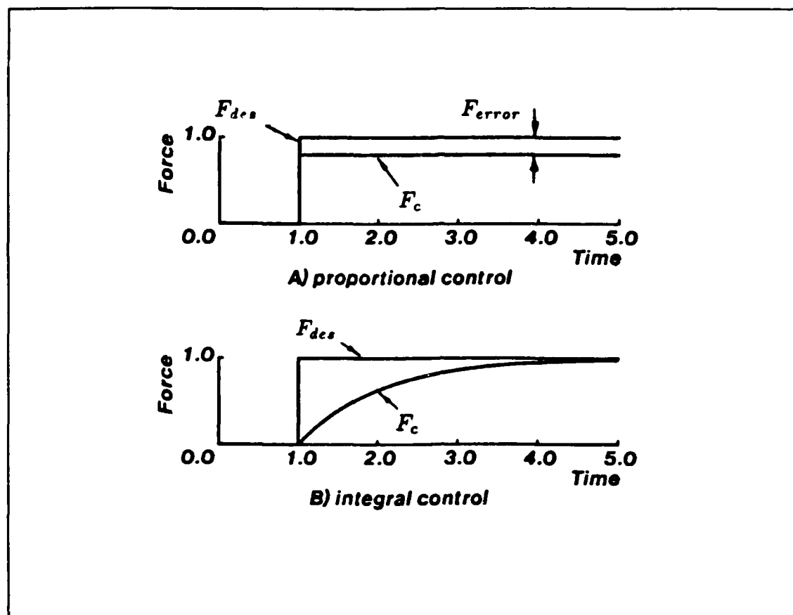
Figure 5.3. Step response with a simple transmission.
