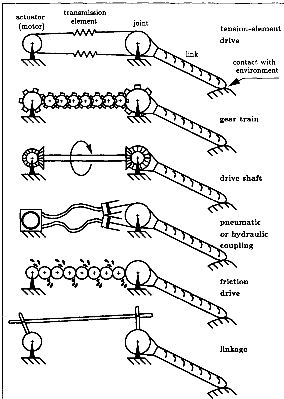
Figure 1.1. Various types of transmissions.
