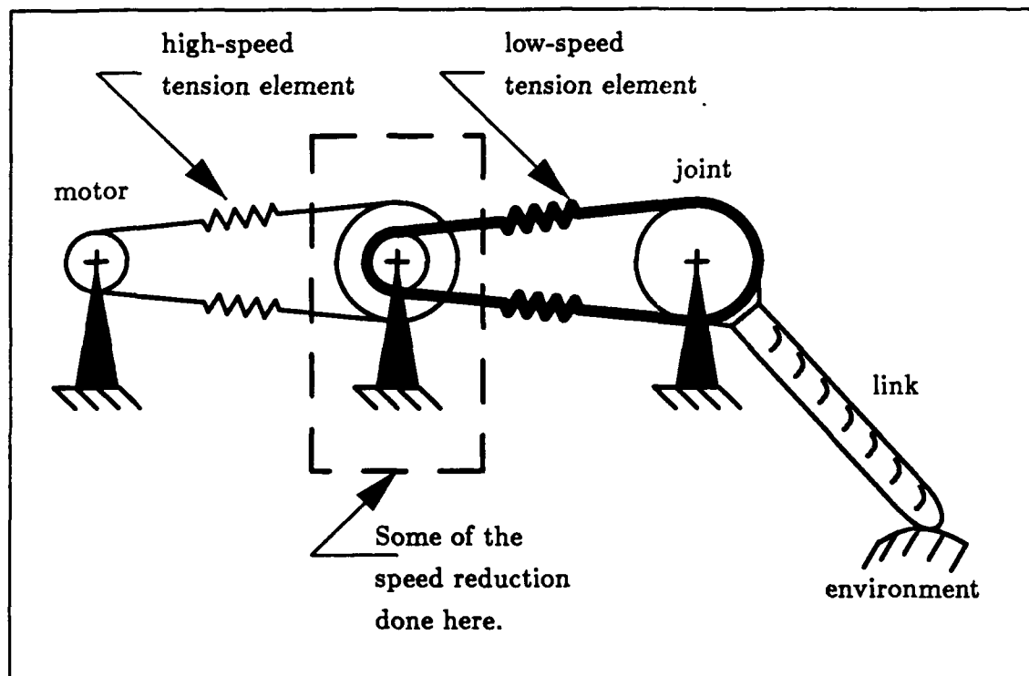
Figure 4.3. Transmission with both integral and distinct reduction.
