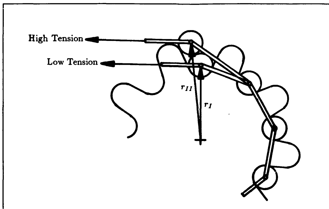
Figure 6.2. The variable radius of chain/sprocket drives.
