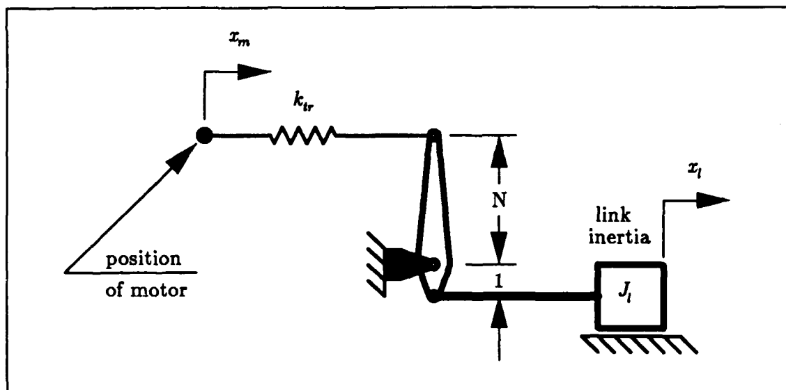
b) Reducer located at joint
