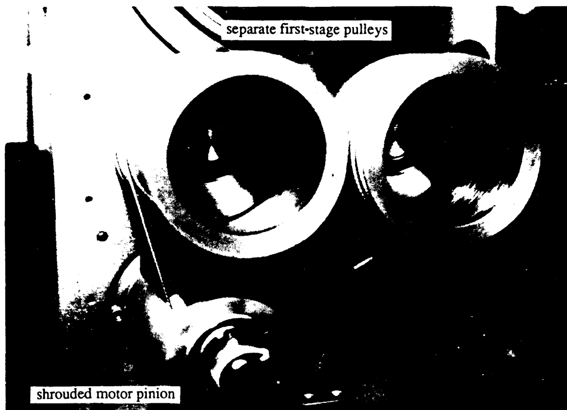
Figure 7 8. Propagated-pretension implementation.
