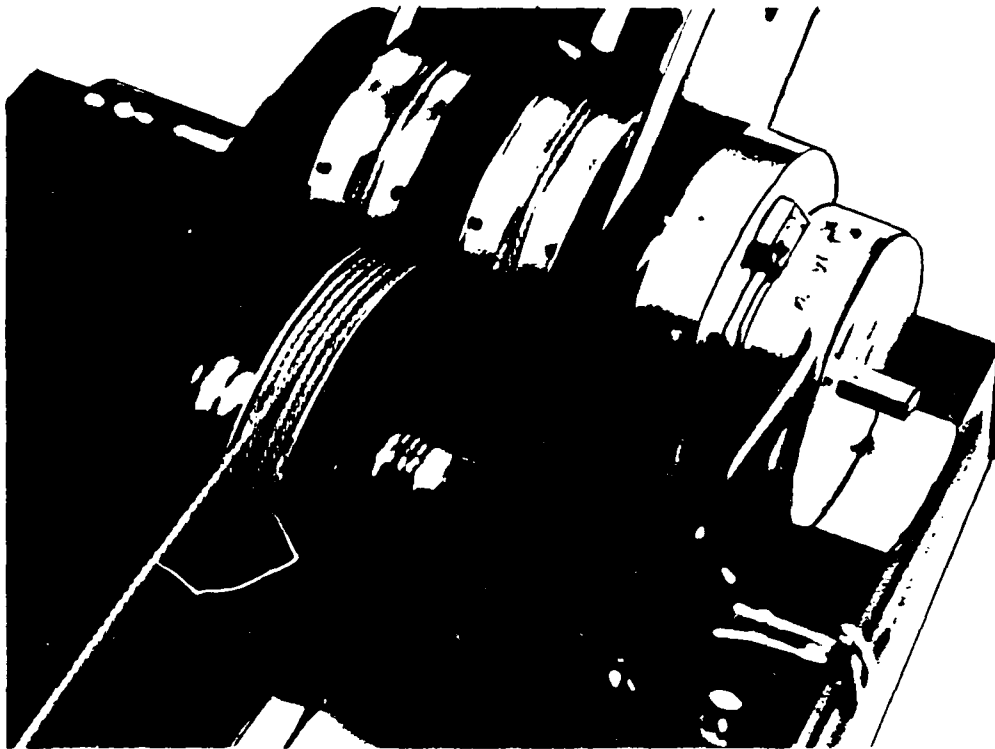
Figure 6.3. Close-up view of two-stage cabled reduction mechanism.
