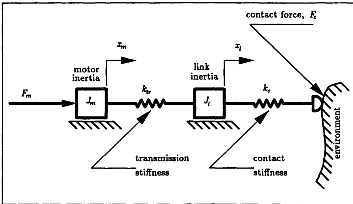
Figure 1.2. Transmission model.
