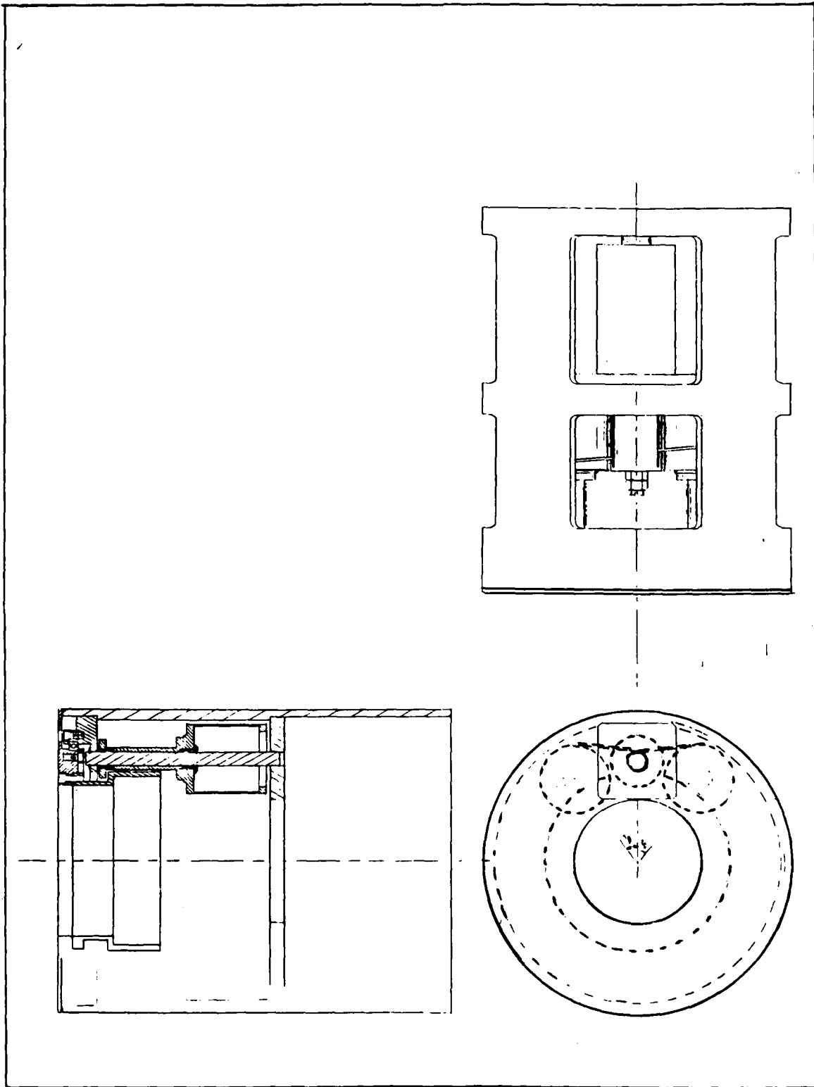
Figure A.5. Assembly drawing of the base.
