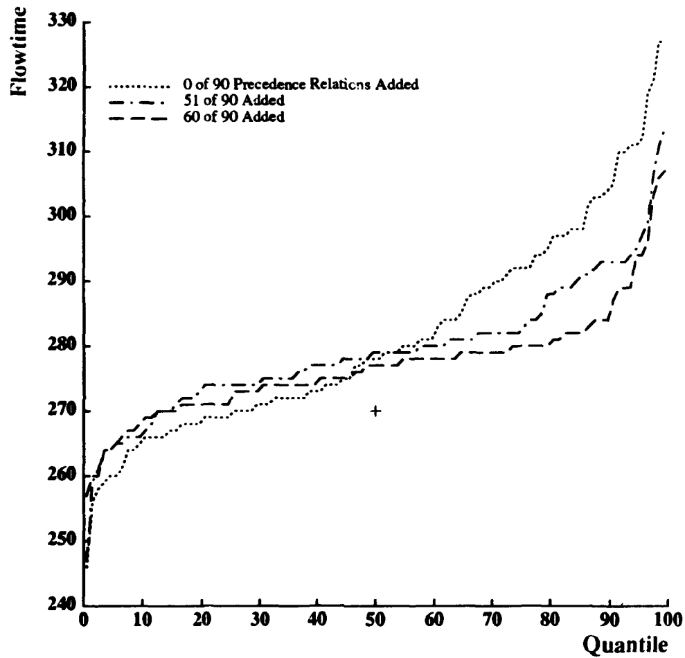
Figure 3.3: H1/CT Applied to a 6 job 6 machine problem
