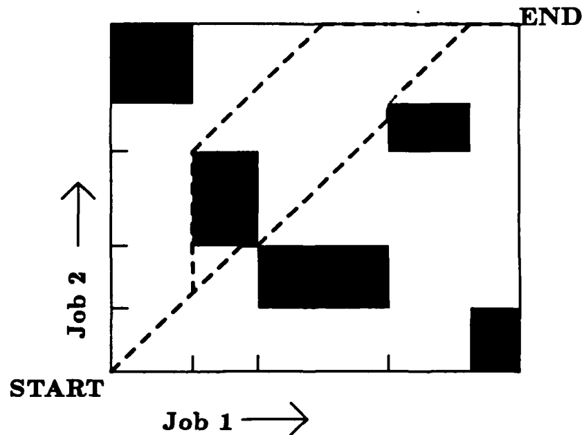
Figure 1.7: Example space associated with a 2 job problem
