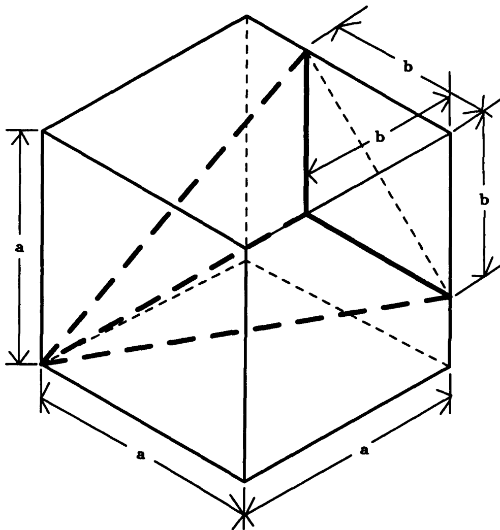
Figure B.1: Three D Cone Example
