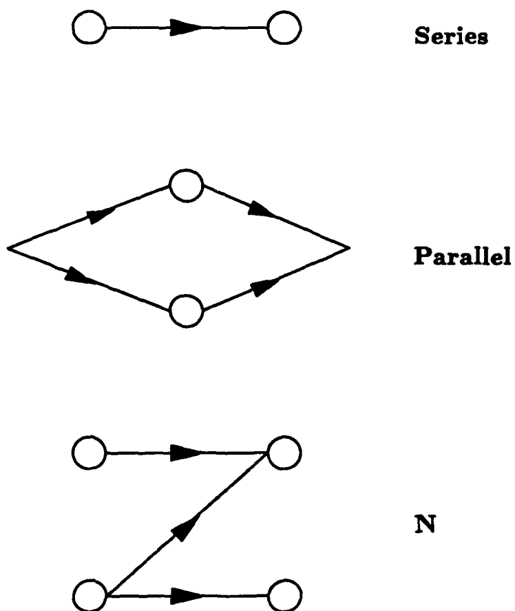
Figure 1.2: AON Series, Parallel and N Subgraphs
