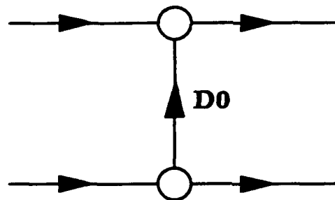
Figure 1.6: AOE Series, Parallel and N Subgraphs
