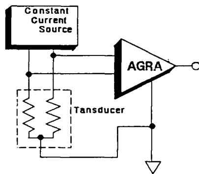
FIGURE 1. CONSTANT CURRENT EXCITATION.
