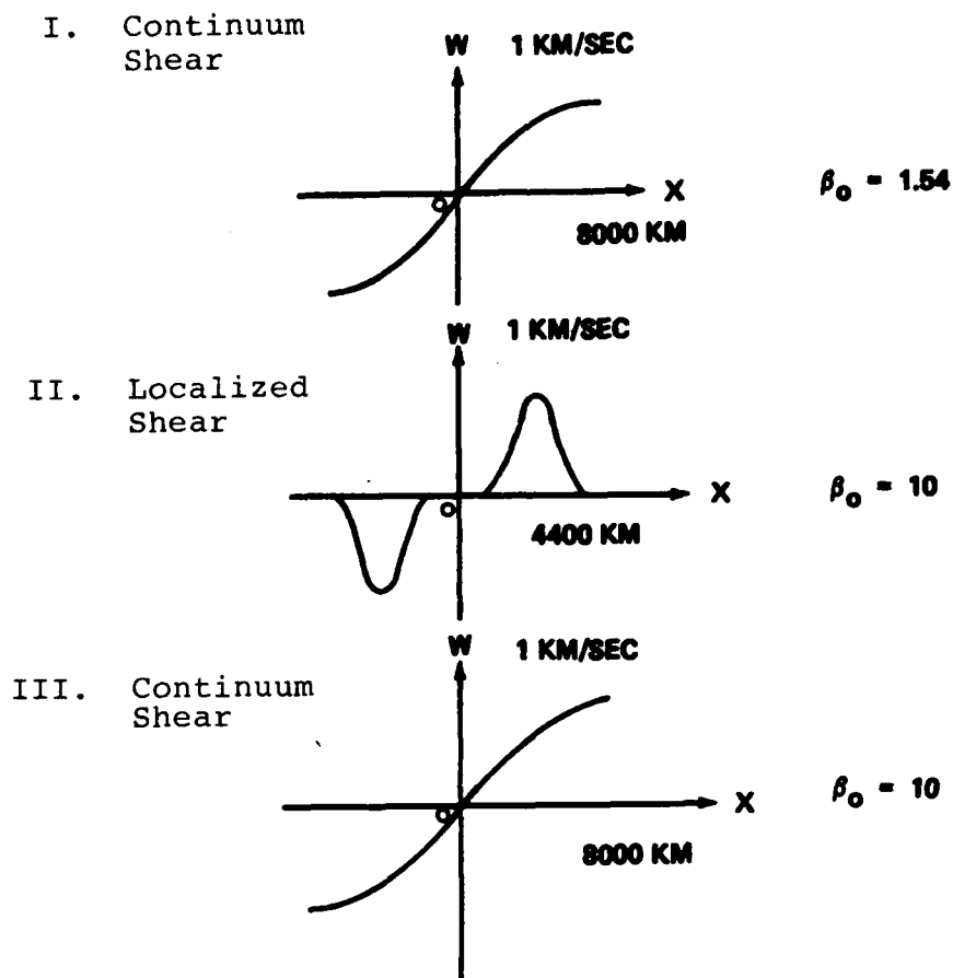
FIGURE III.2. Schematic Representation of the Prescribed Perturbations, i.e., the Configuration of Shear Motion Input to the MHD Model for a Specified Initial \beta_0 .
