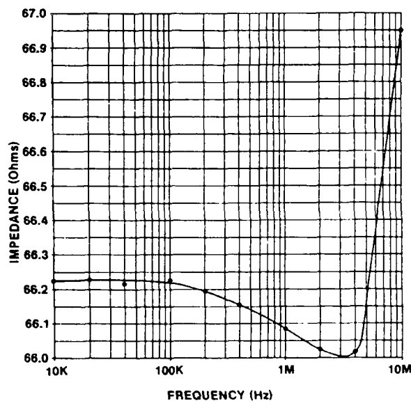
FIGURE 6: MEASURED IMPEDANCE-VS-FREQUENCY FOR CYLINDRICAL SAMPLE OF GRAPHITE IN POLYCARBONATE (@.1V)
