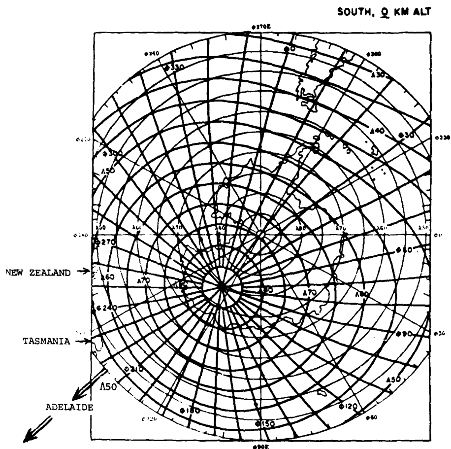
Figure 3. Invariant Geomagnetic Co-ordinates, Epoch 1969.75 (from Evans et al (1969), Ref. 28).
