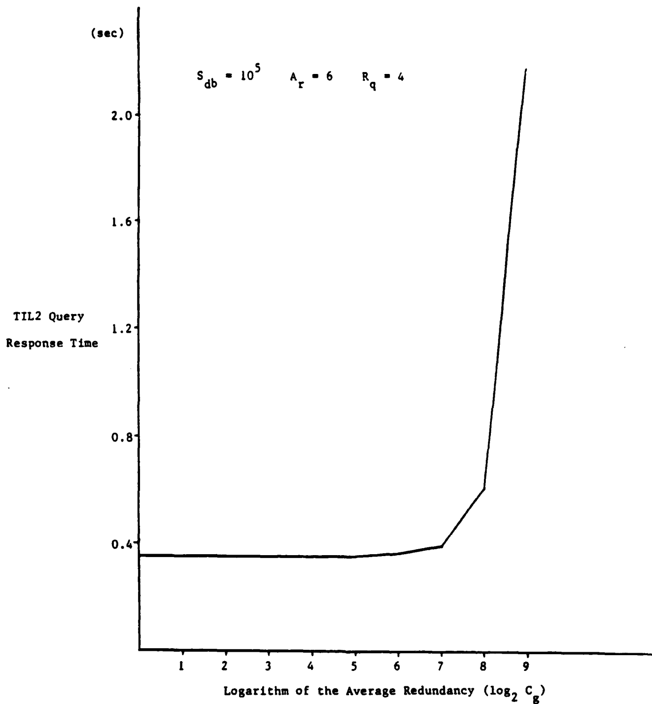
Figure 9.26 TIL2 Query Response Time ( S_{db} = 10^5 bytes, A_r = 6 , R_q = 4 )
