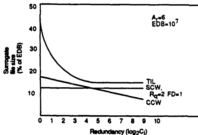
Figure 5. Surrogate file size comparison.
