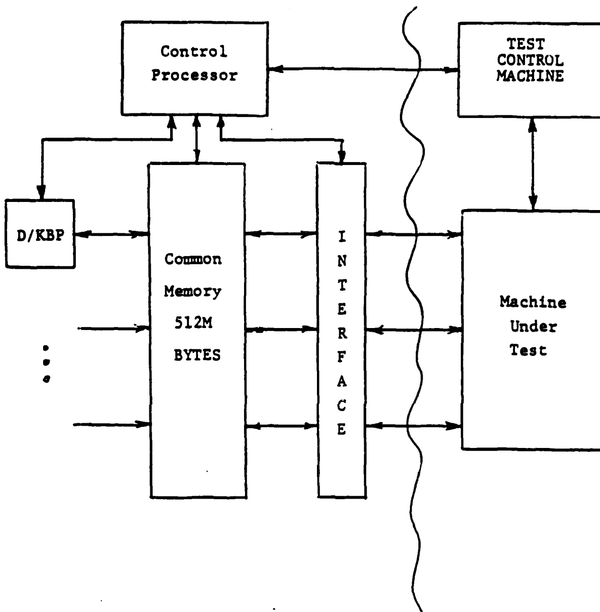
Figure 3. KBSA Configured for Machine Evaluation
