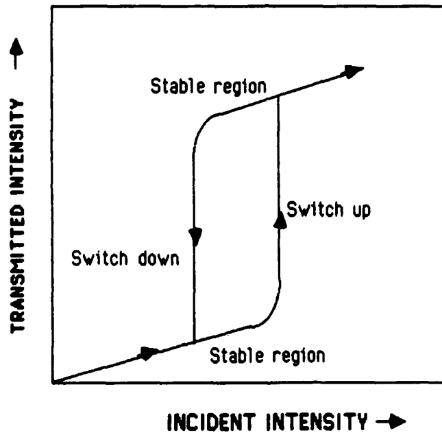
Fig. 5 Effect of a non-linear material in a Fabry-Perot cavity
