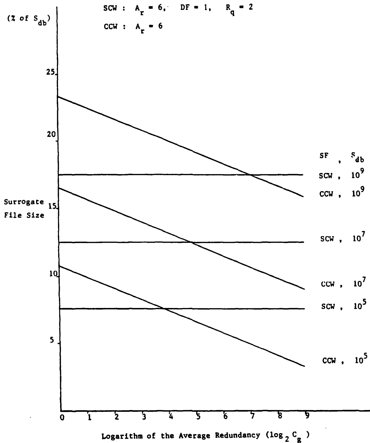
Figure 5.5 SCW and CCW Surrogate File Size Comparison
