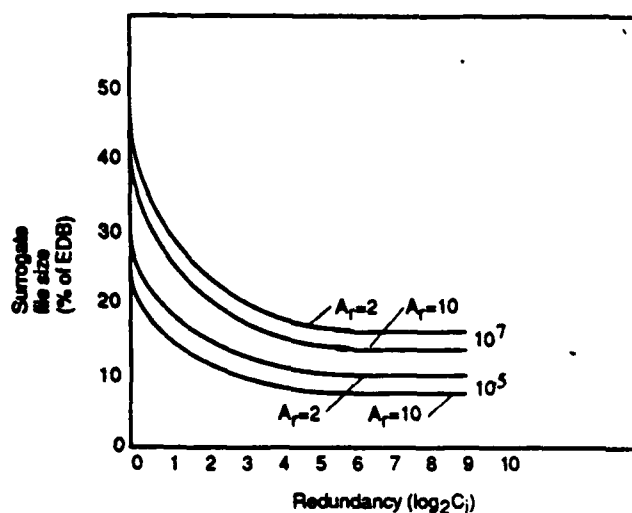
Figure 4. Surrogate file size for TIL.
