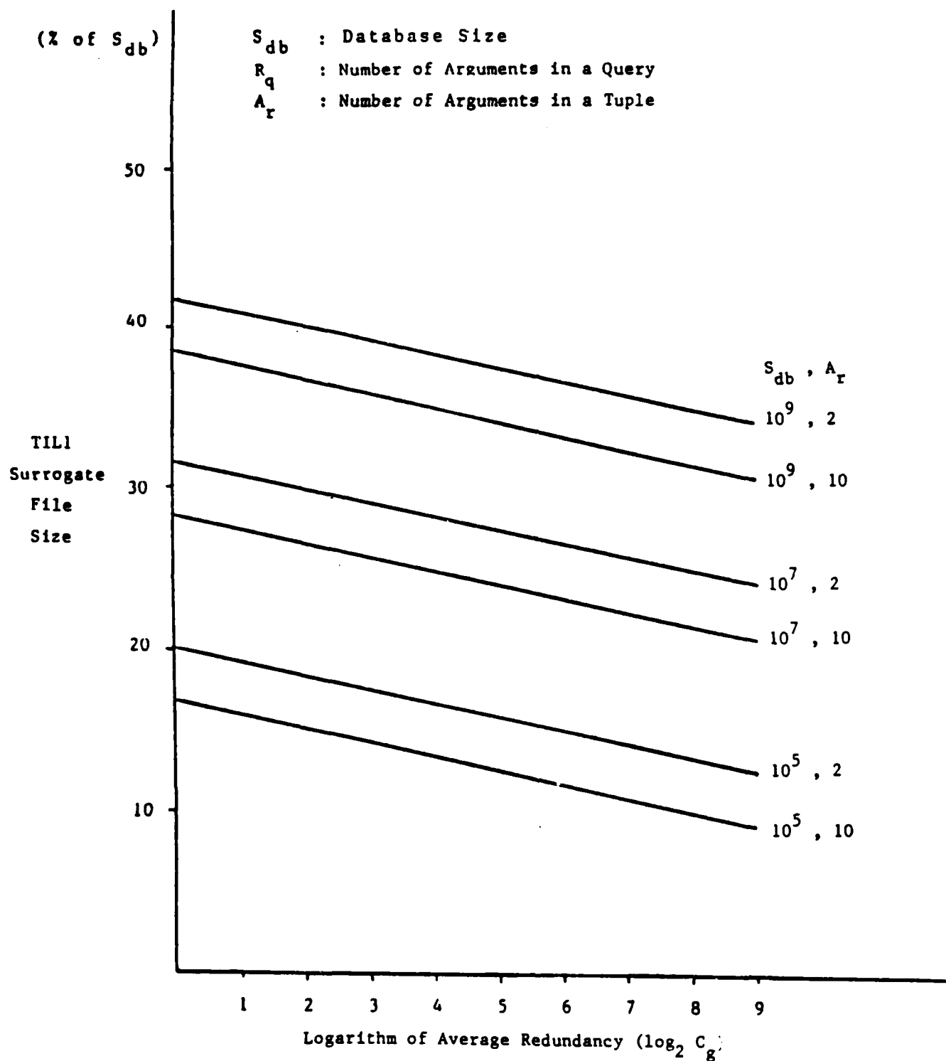
Figure 9.1 Effect of the DB Size and the Number of Arguments in a Tuple on the TIL1 Surrogate File Size.
