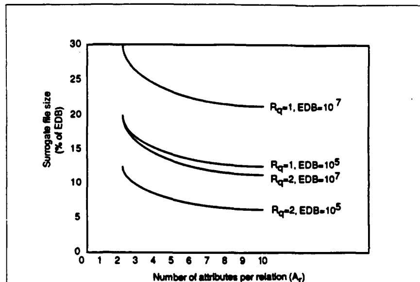
Figure 2. Surrogate file size for SCW.
