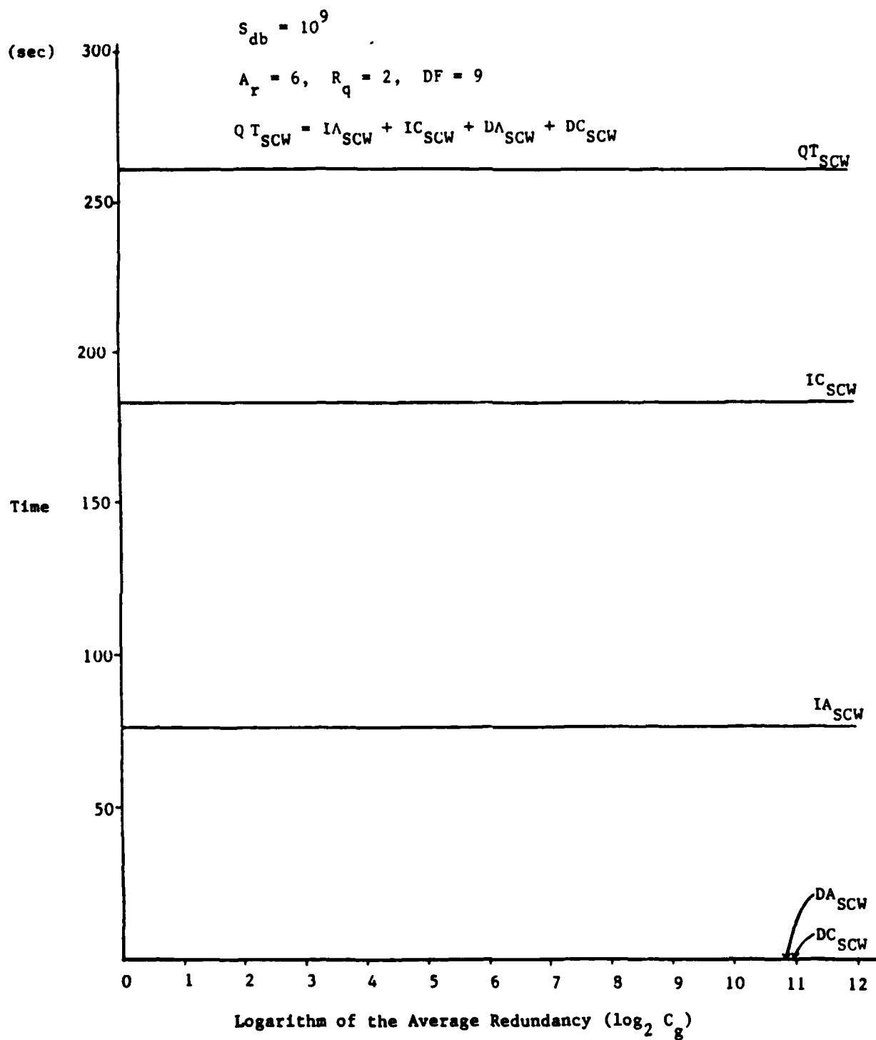
Figure 5.8 Components of the SCW Query Response Time ( S_{db} = 10^9 bytes)
