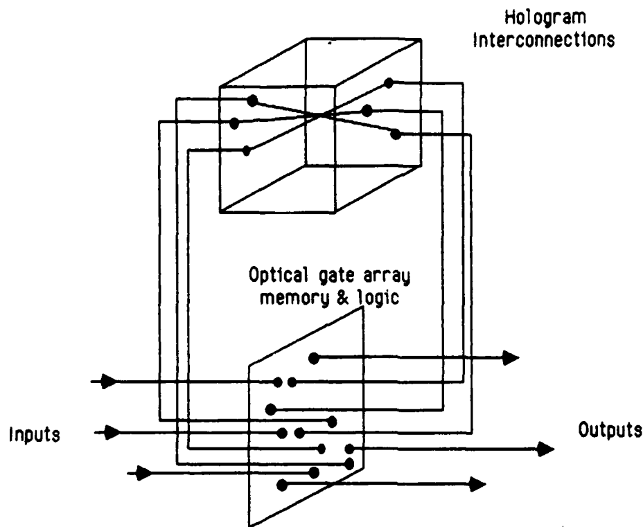
Fig. 9 Free-Interconnection non von Neumann processor
