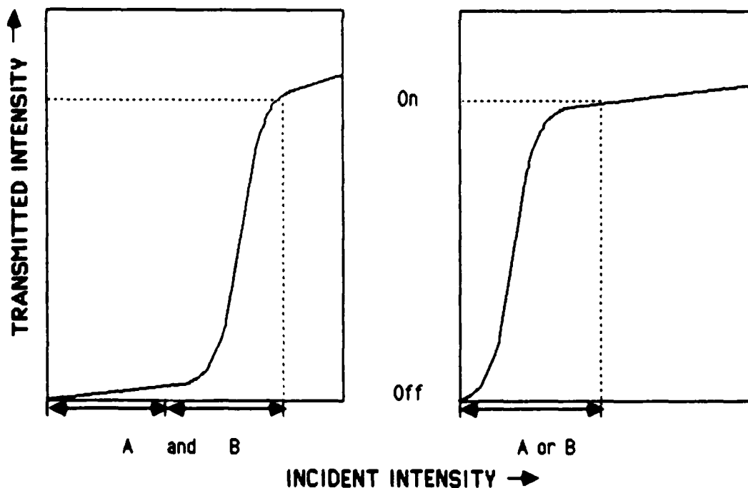
Fig. 6 Implementing Boolean Connectives
