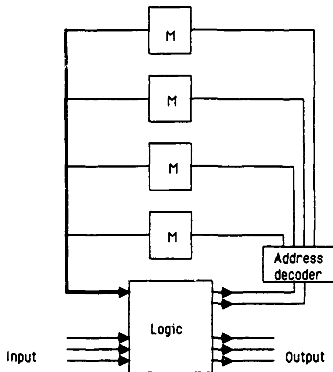
Fig. 7 Finite State Machine v. Von Neumann bottleneck
