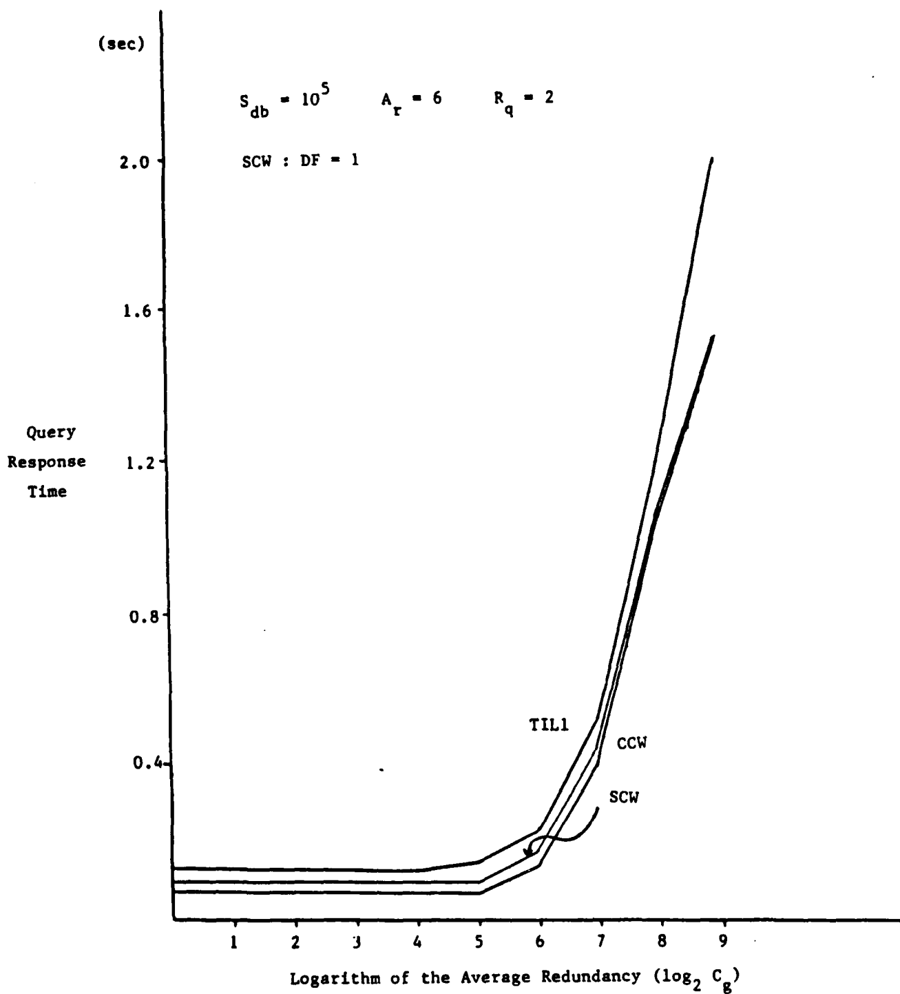
Figure 10.4 Query Response Time Comparison ( S_{db} = 10^5 bytes)
