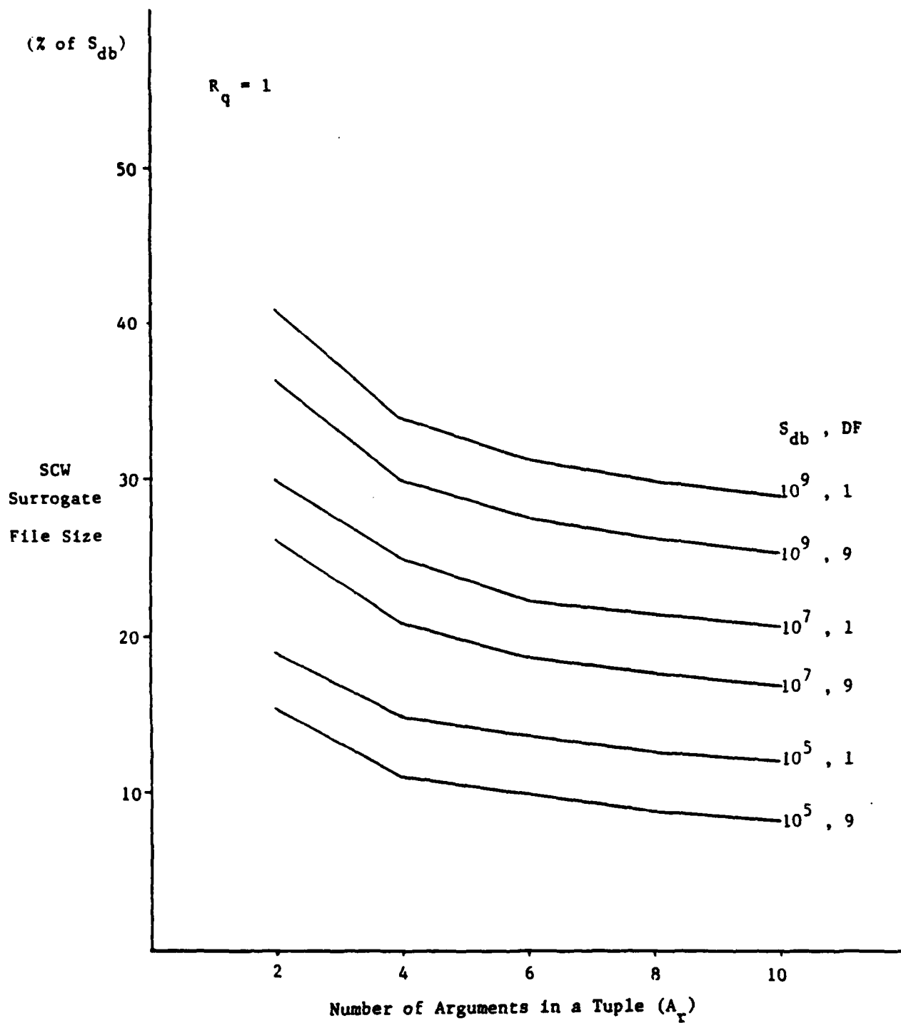
Figure 5.2 Effect of False Drops on the SCW Surrogate File Size
