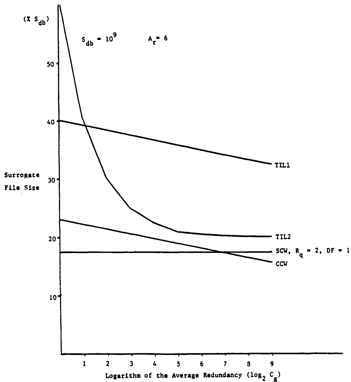
Figure 10.3 Surrogate File Size Comparison ( S_{db} = 10^9 bytes)
