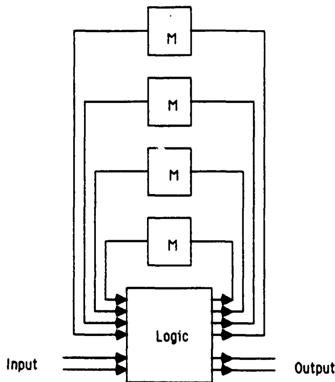
Fig. 8 Classic Finite State Machine
