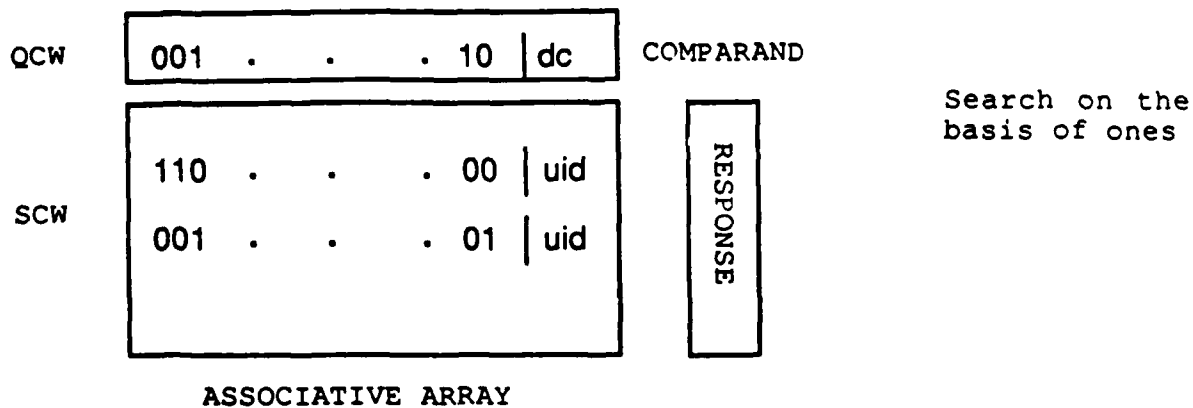
Figure 11.1.a SCW Mapped into Associative Memory
