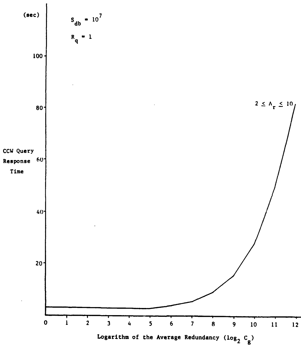
Figure 5.16 Effect of the Number of Arguments in a Tuple on the CCW Query Response Time ( S_{db} = 10^7 bytes)
