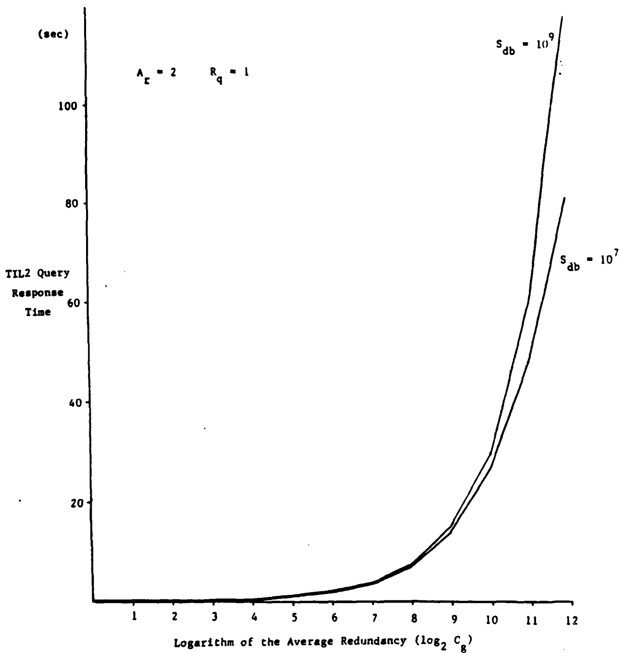
Figure 9.25 TIL2 Query Response Time ( S_{db} = 10^7 and 10^9 bytes, R_q = 1 )
