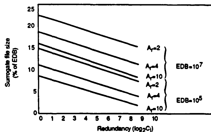
Figure 3. Surrogate file size for CCW.
